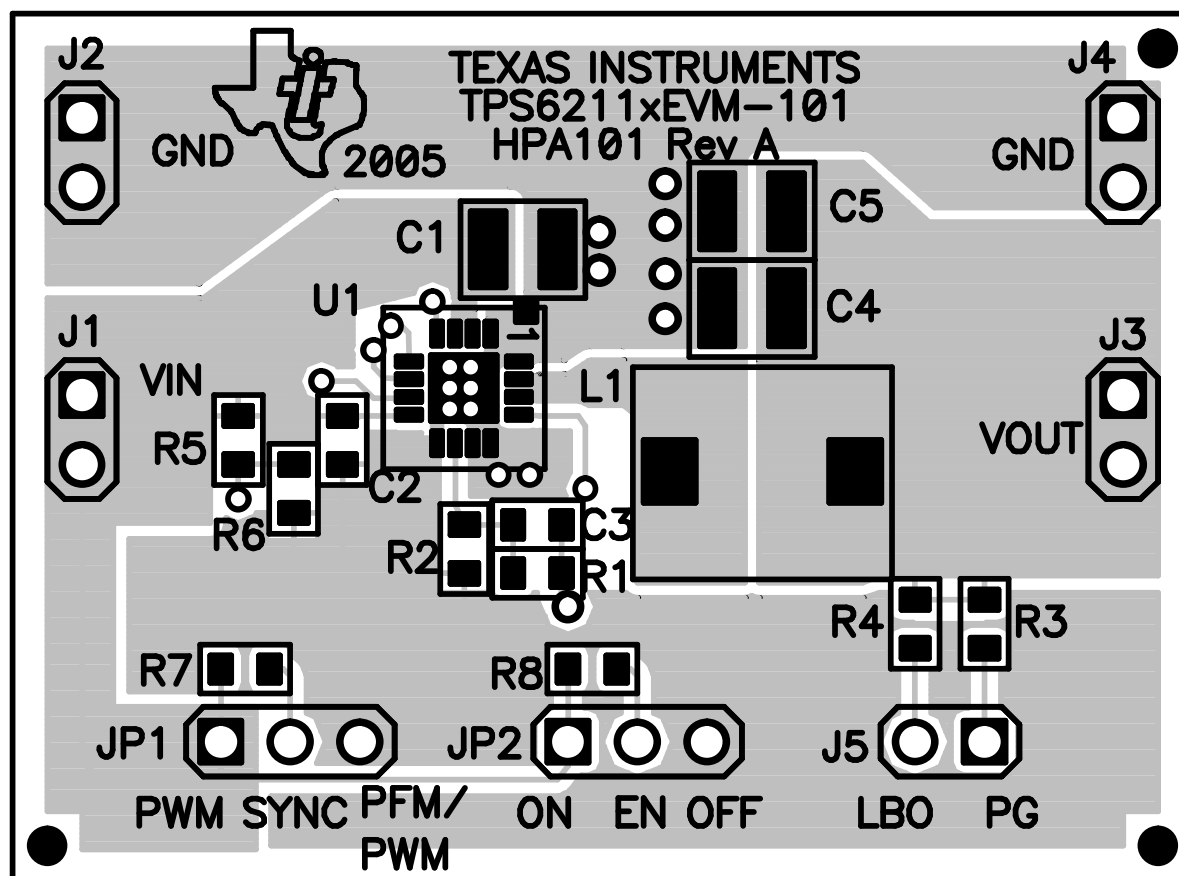
Figure 1. Assembly Layer
