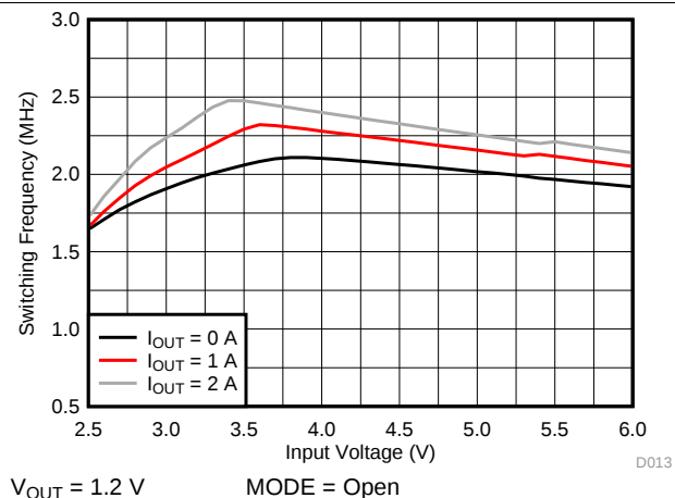
Figure 19. Switching Frequency, Forced PWM Mode (2.5MHz)
