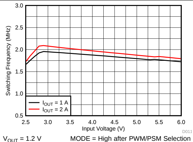
Figure 17. Switching Frequency, Forced PWM Mode (2.0MHz)
