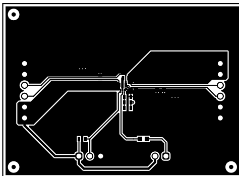
Figure 3. Top Layer
