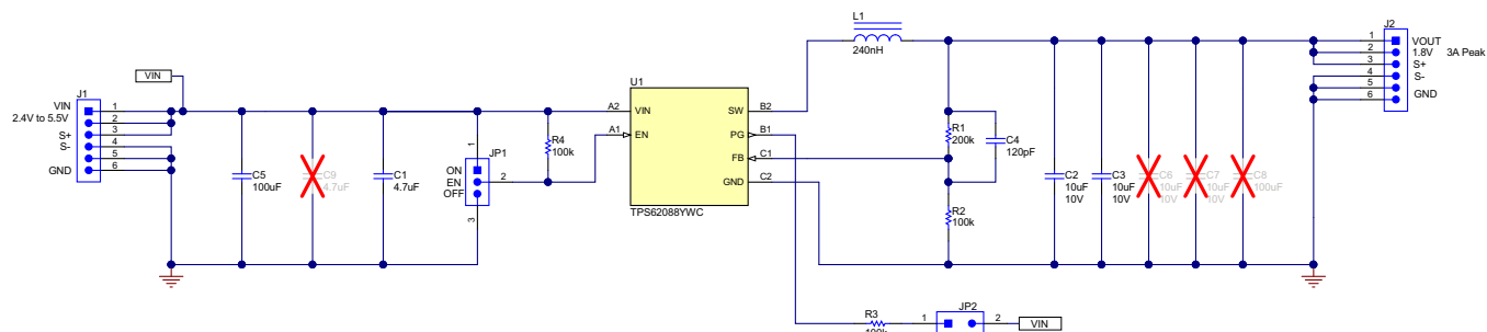
Figure 9. TPS62088YWCEVM-084 Schematic
