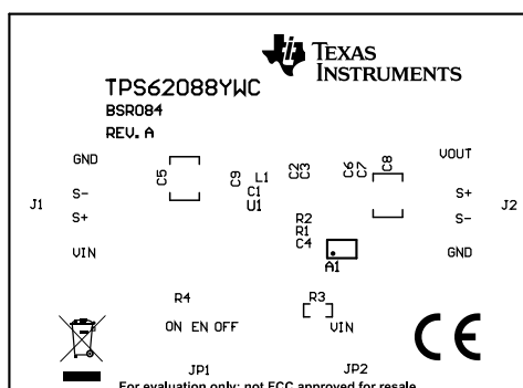
Figure 2. Top Assembly
