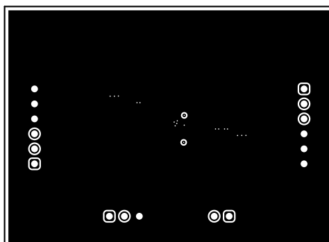
Figure 4. Signal Layer 1
