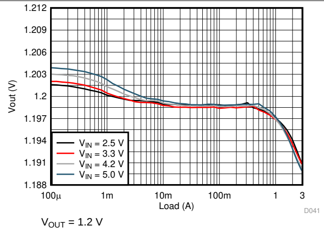
Figure 12. Load Regulation
