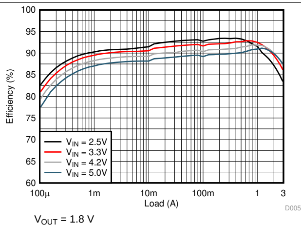
Figure 13. Efficiency
