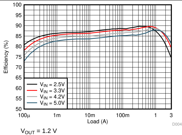
Figure 11. Efficiency
