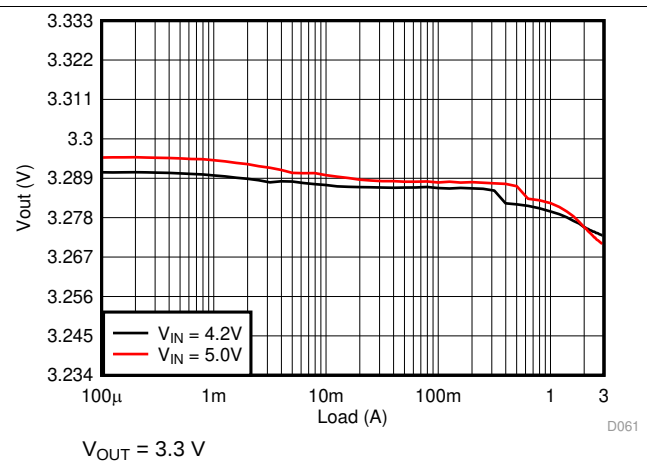
Figure 16. Load Regulation
