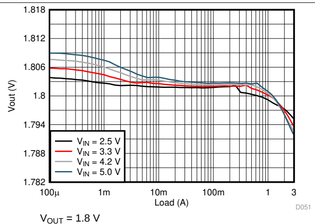
Figure 14. Load Regulation
