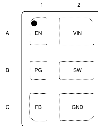
YWC Package Top View
