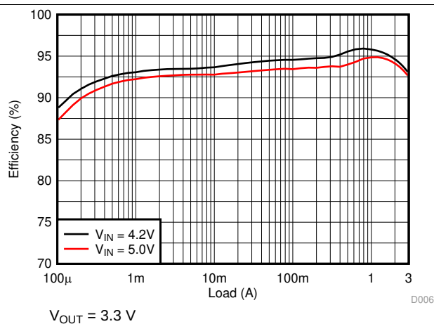
Figure 15. Efficiency
