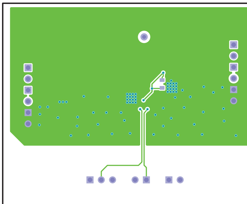
Figure 7. Bottom Layer
