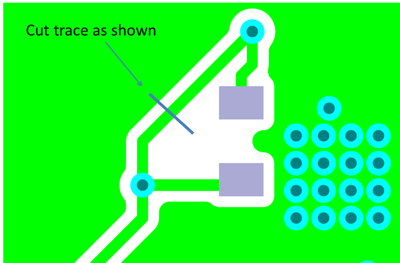
Figure 1. Loop Response Measurement Modification
