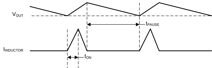
Figure 2. Power Save Mode Waveform Diagram
