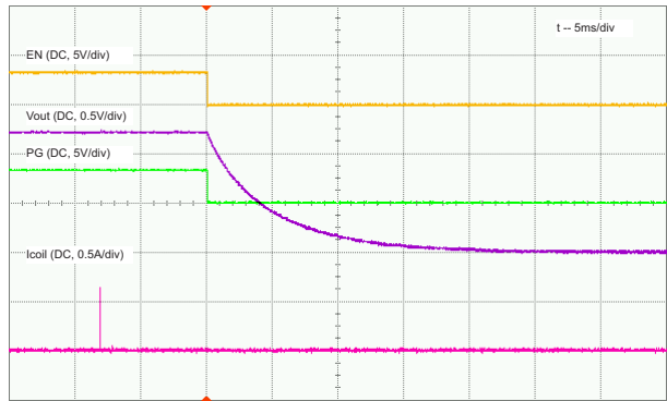
Figure 16. Shutdown, Load = Open
