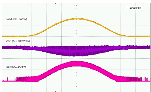
Figure 10. PWM Operation, Load = 3 A
