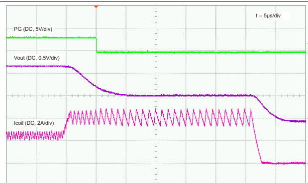
Figure 19. Output Short-Circuit Protection, Load = 0.47 \Omega , Entry
