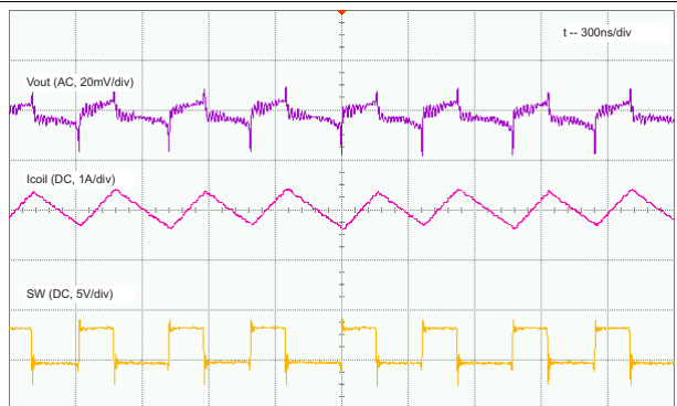
Figure 10. PWM Operation, Load = 3 A
