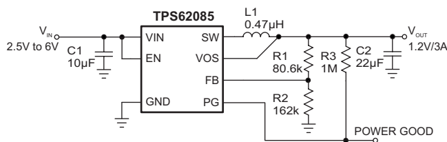
Figure 3. 1.2-V Output Voltage Application
