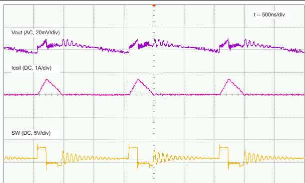
Figure 11. PSM Operation, Load = 100 mA
