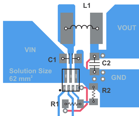
Figure 22. PCB Layout Recommendation
