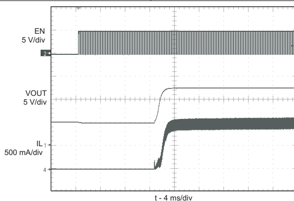
Figure 10. Analog Dimming Start-up
