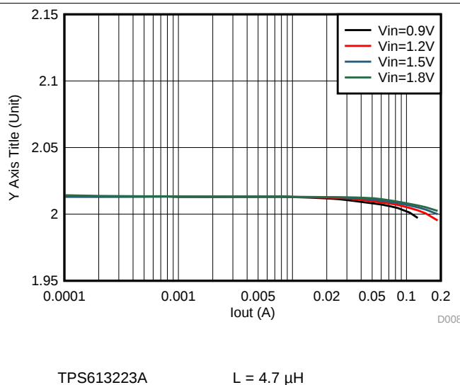
Figure 10. Load Regulation
