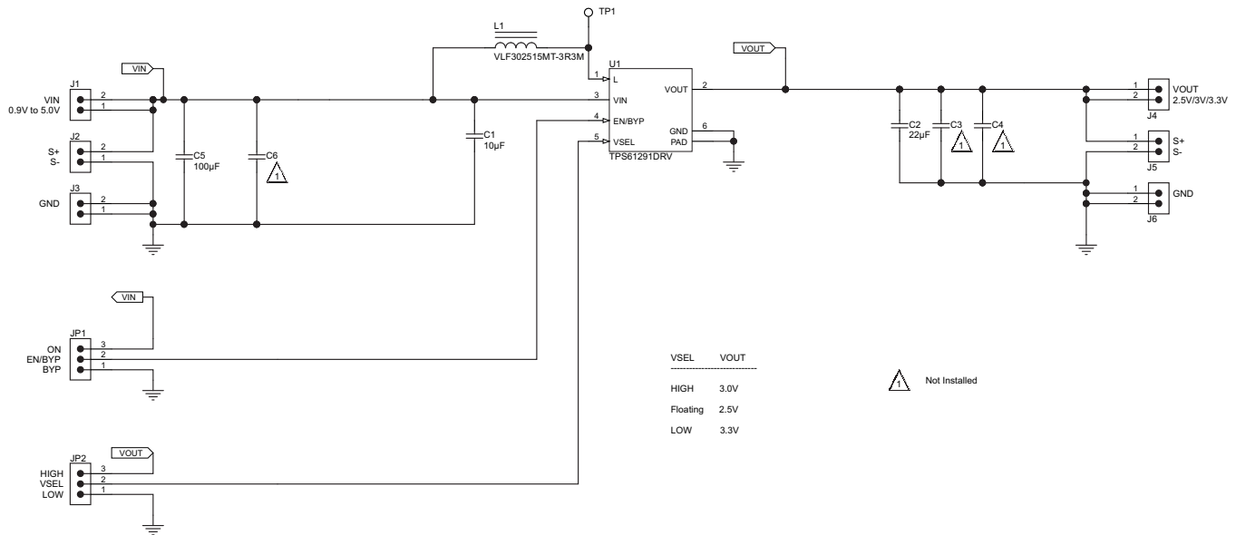
Figure 5. TPS61291EVM-569 Schematic
