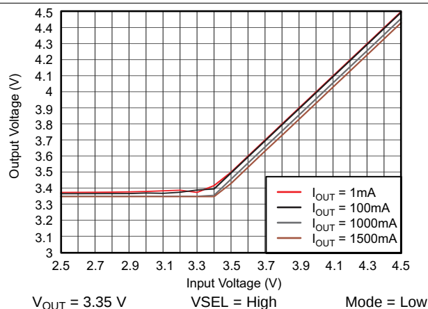
Figure 44. TPS61281D DC Output Voltage vs Input Voltage
