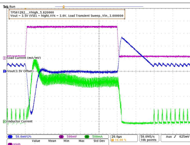
Figure 70. TPS61282D Load Transient Response In PFM/PWM Operation
