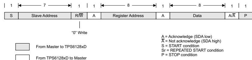
Figure 24. : “Write” Data Transfer Format in Standard-, Fast, Fast-Plus Modes
