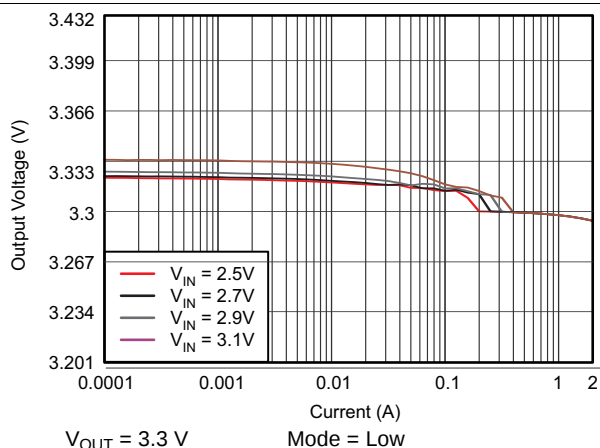
Figure 59. TPS61280D DC Output Voltage vs Output Current
