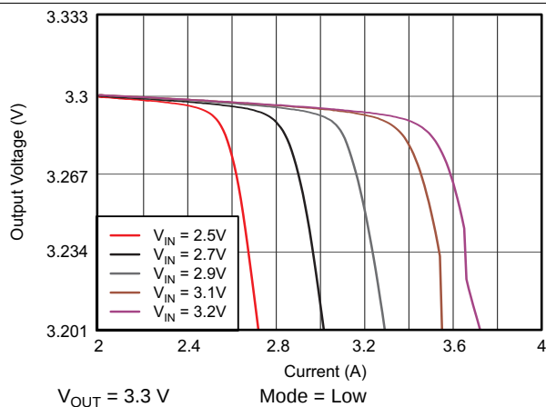
Figure 60. TPS61280D DC Output Voltage vs Output Current
