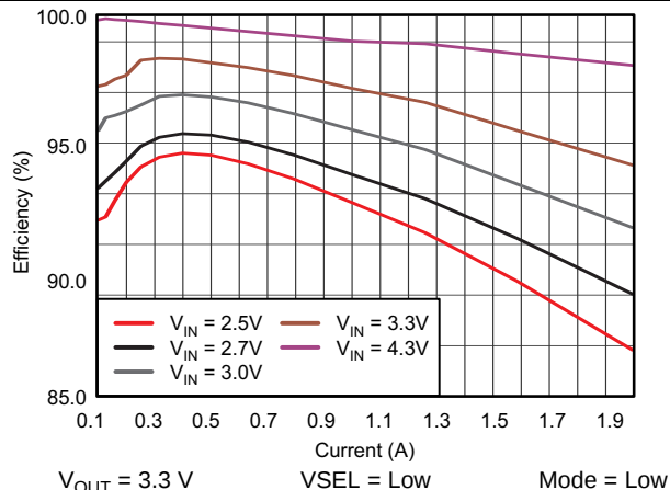
Figure 56. TPS61280D Efficiency vs Output Current
