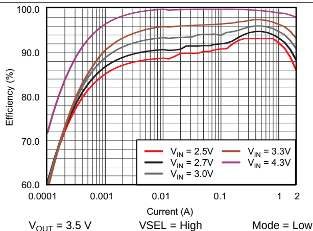
Figure 57. TPS61280D Efficiency vs Output Current
