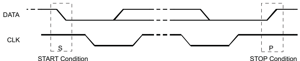
Figure 20. START and STOP Conditions
