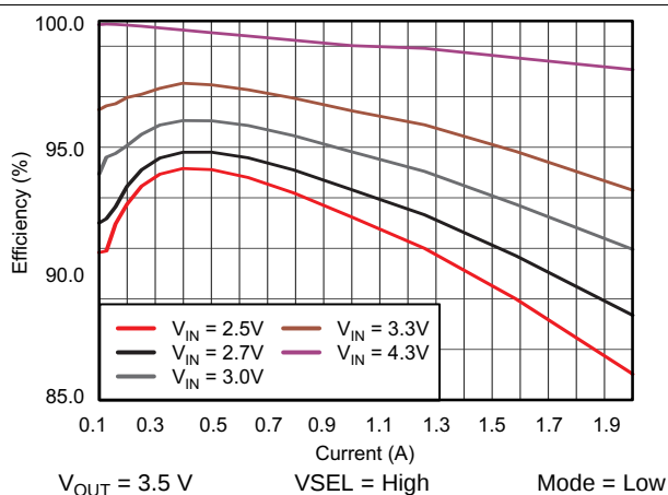
Figure 58. TPS61280D Efficiency vs Output Current
