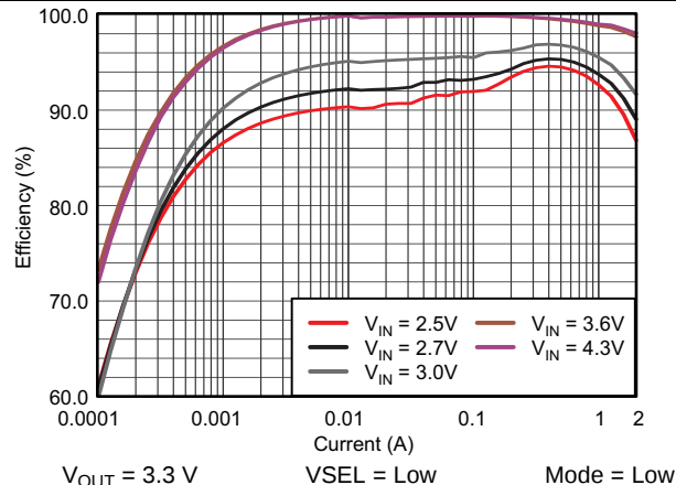
Figure 55. TPS61280D Efficiency vs Output Current
