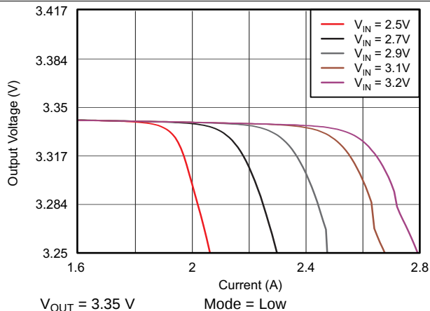
Figure 42. TPS61281D DC Output Voltage vs Output Current
