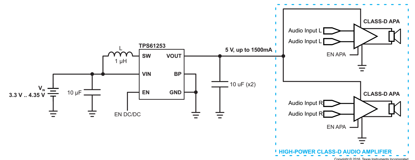
Figure 38. "Boosted" Stereo Audio Power Supply
