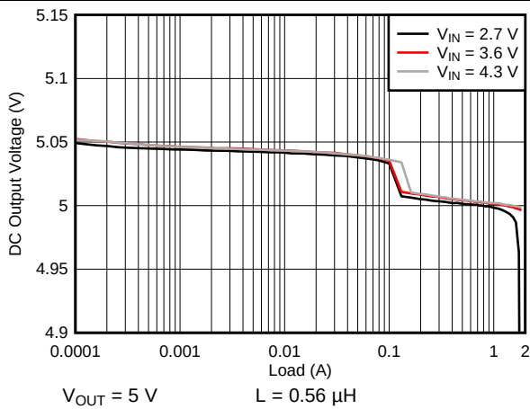
Figure 3. DC Output Voltage vs Load
