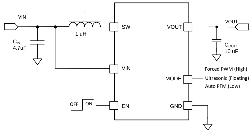
Figure 31. Typical Application with Minimum Output Capacitance
