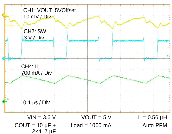
Figure 24. Steady 1000 mA
