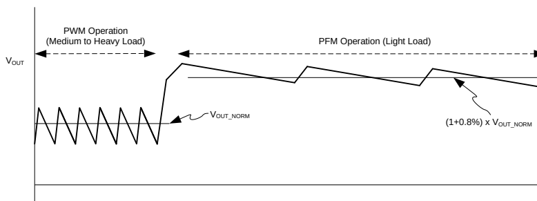
Figure 20. Output Voltage in Auto PFM / PWM Mode
