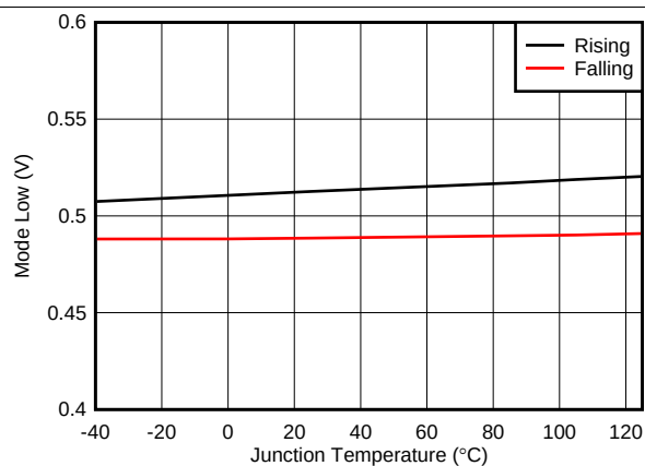
Figure 14. Mode Low Rising / Falling vs Temperature
