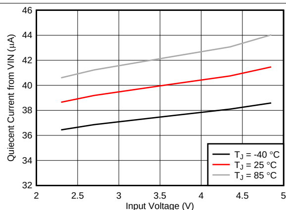
Figure 7. Quiescent Current (from VIN) vs Input Voltage
