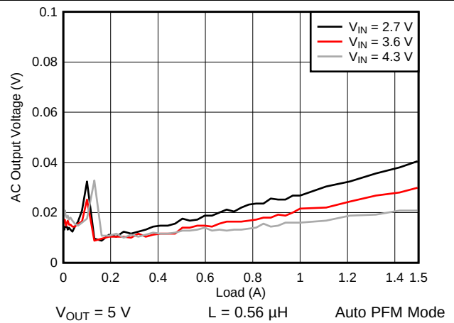
Figure 4. AC Output Voltage vs Load
