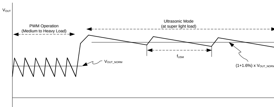
Figure 21. Ultrasonic Mode Operation
