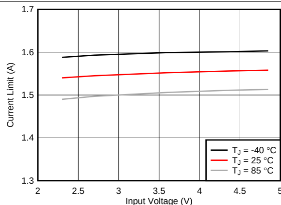
Figure 10. Current Limit (Auto PFM) vs Input Voltage
