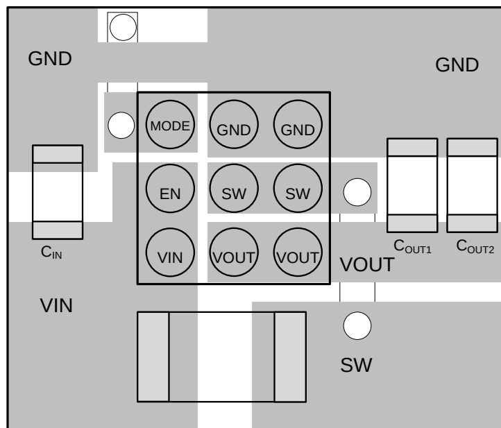
Figure 32. Recommended Layout
