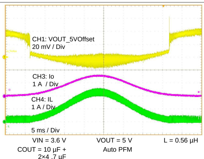
Figure 26. Load Sweep
