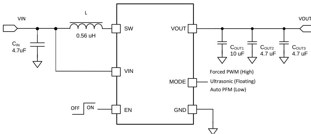
Figure 22. Typical Application Circuit
