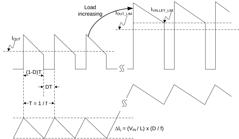
Figure 18. Current Limit Operation
