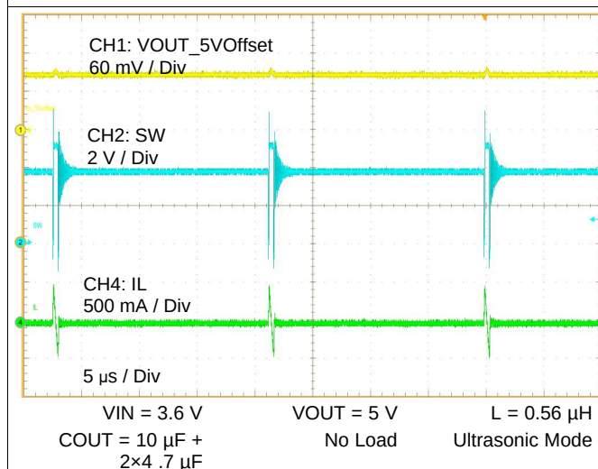
Figure 25. Steady Ultrasonic Mode
