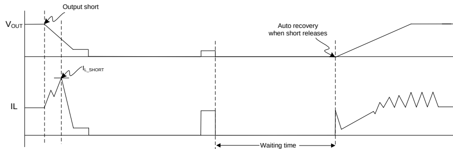
Figure 19. Hiccup Mode Short Protection
