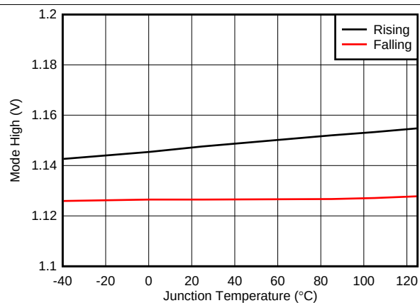
Figure 13. Mode High Rising / Falling vs Temperature
