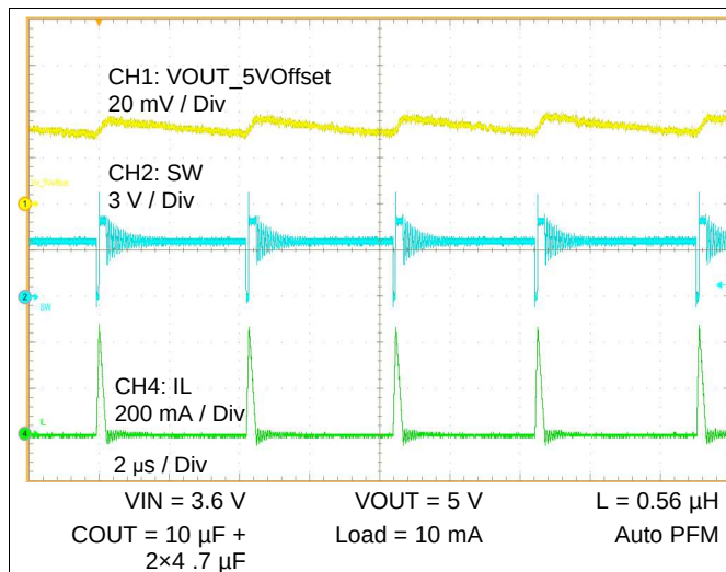
Figure 23. Steady 10 mA
