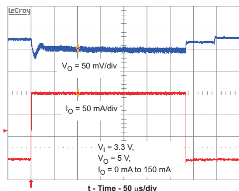
Figure 4. TPS61252 EVM Load Transient Response with Mode Change, Snooze Mode to Pulse Frequency Mode
