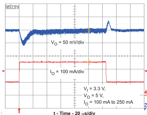
Figure 3. TPS61252 EVM Load Transient Response Continuous Conduction Mode
