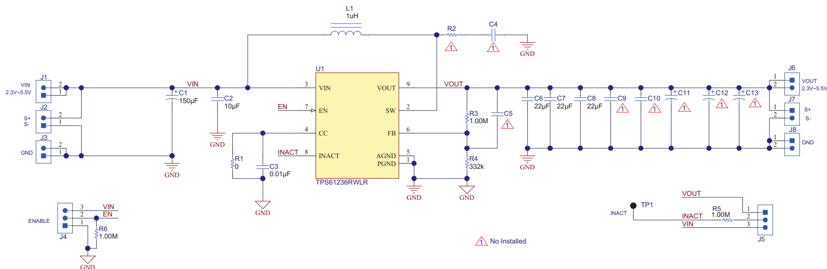
Figure 1. TPS61236EVM Schematic
