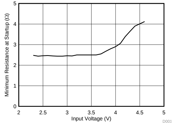
Figure 8. Minimum Load Resistance at Startup
