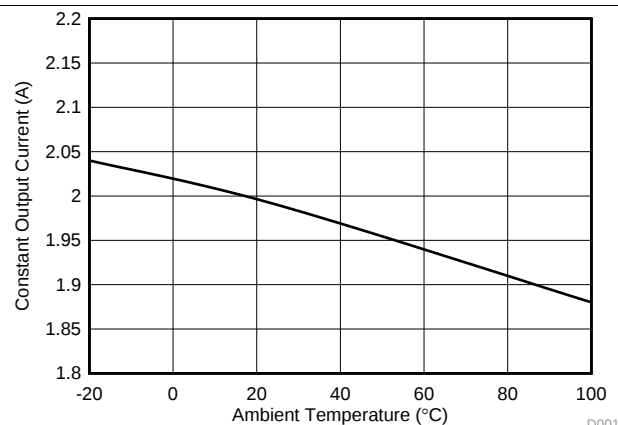
Figure 10. Current Limit vs Ambient Temperature
