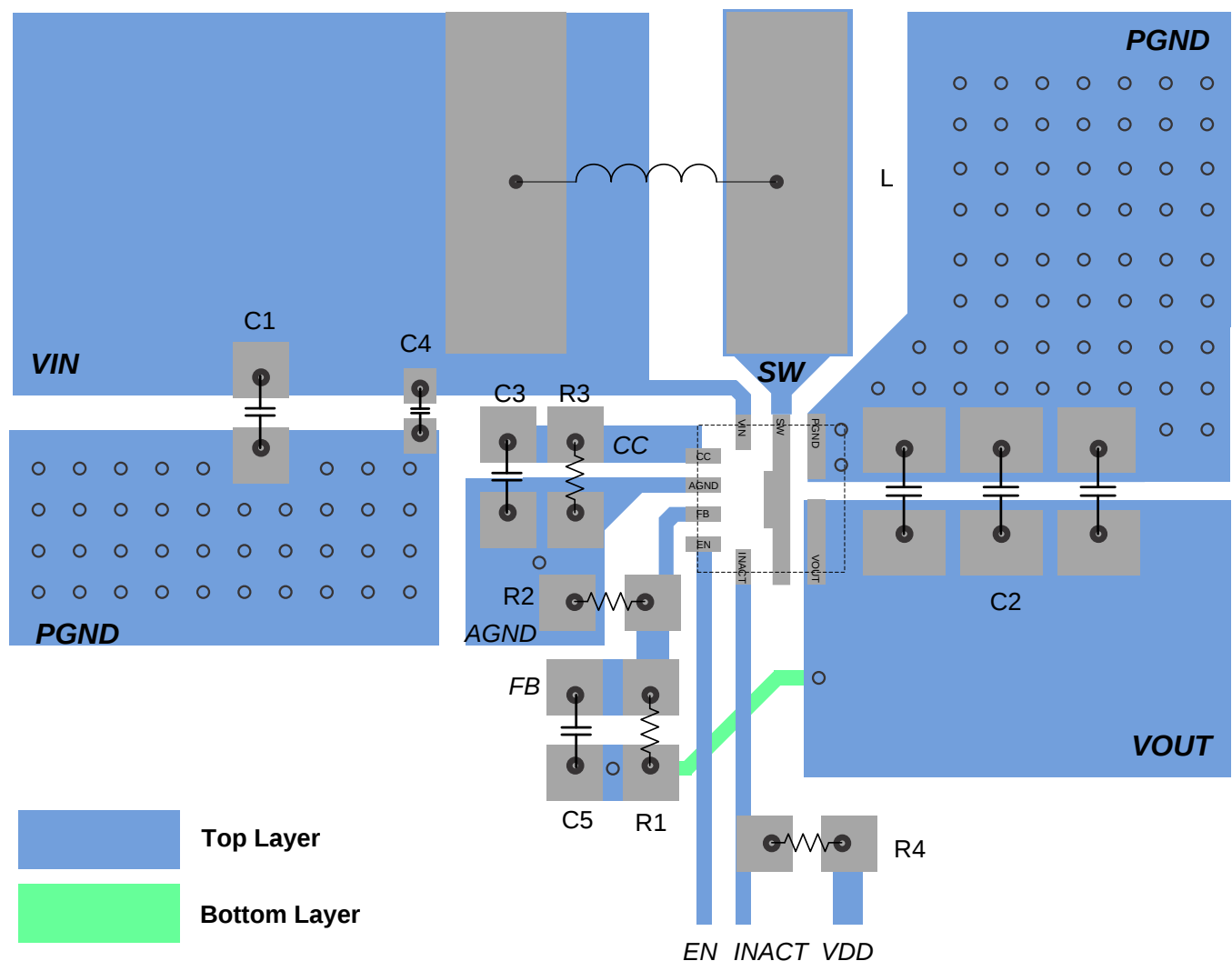
Figure 39. Layout Recommendation
