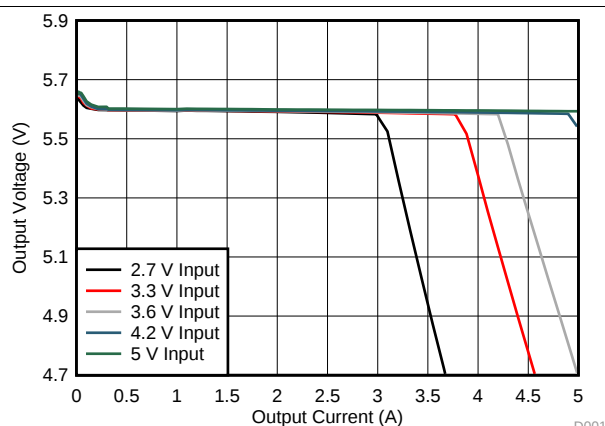
Figure 35. Load Regulation
