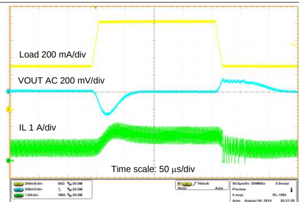
Figure 19. Load Sweep
