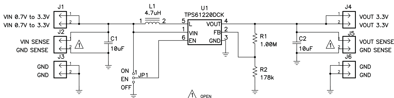
Figure 4. TPS61220EVM-319 Schematic
