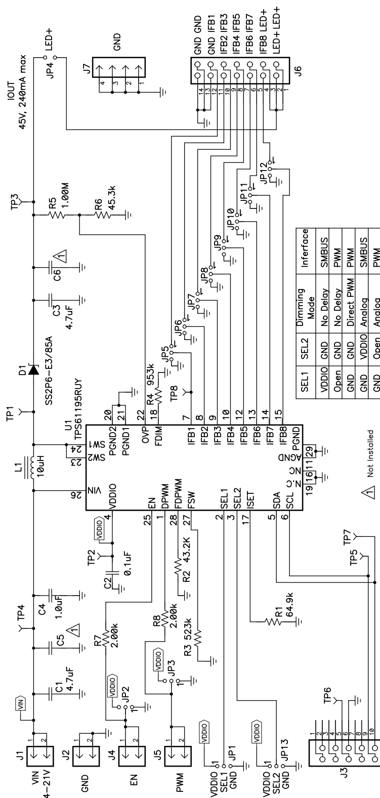
Figure 1. HPA460EVM Schematic
