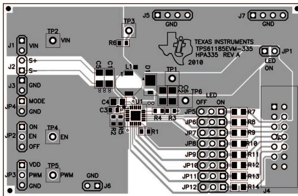
Figure 3. TPS61185EVM-335 Top Copper, Viewed From Top
