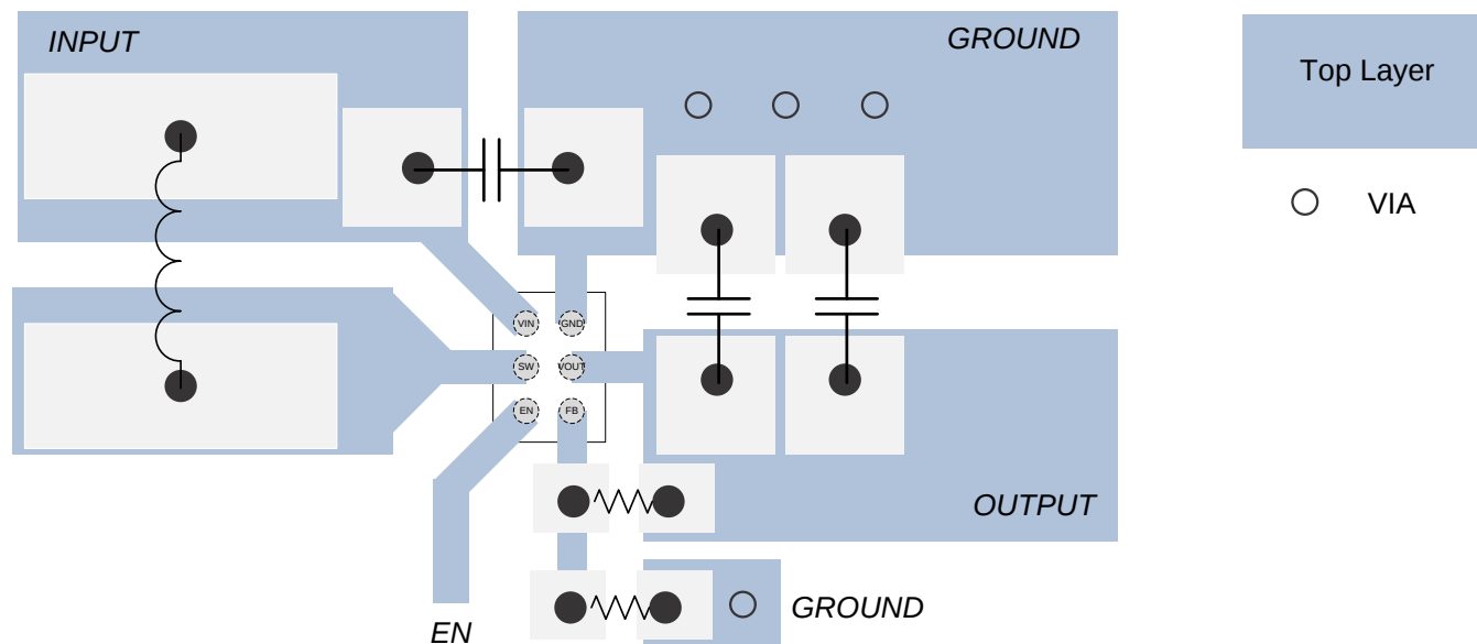
Figure 29. Layout -YFF
