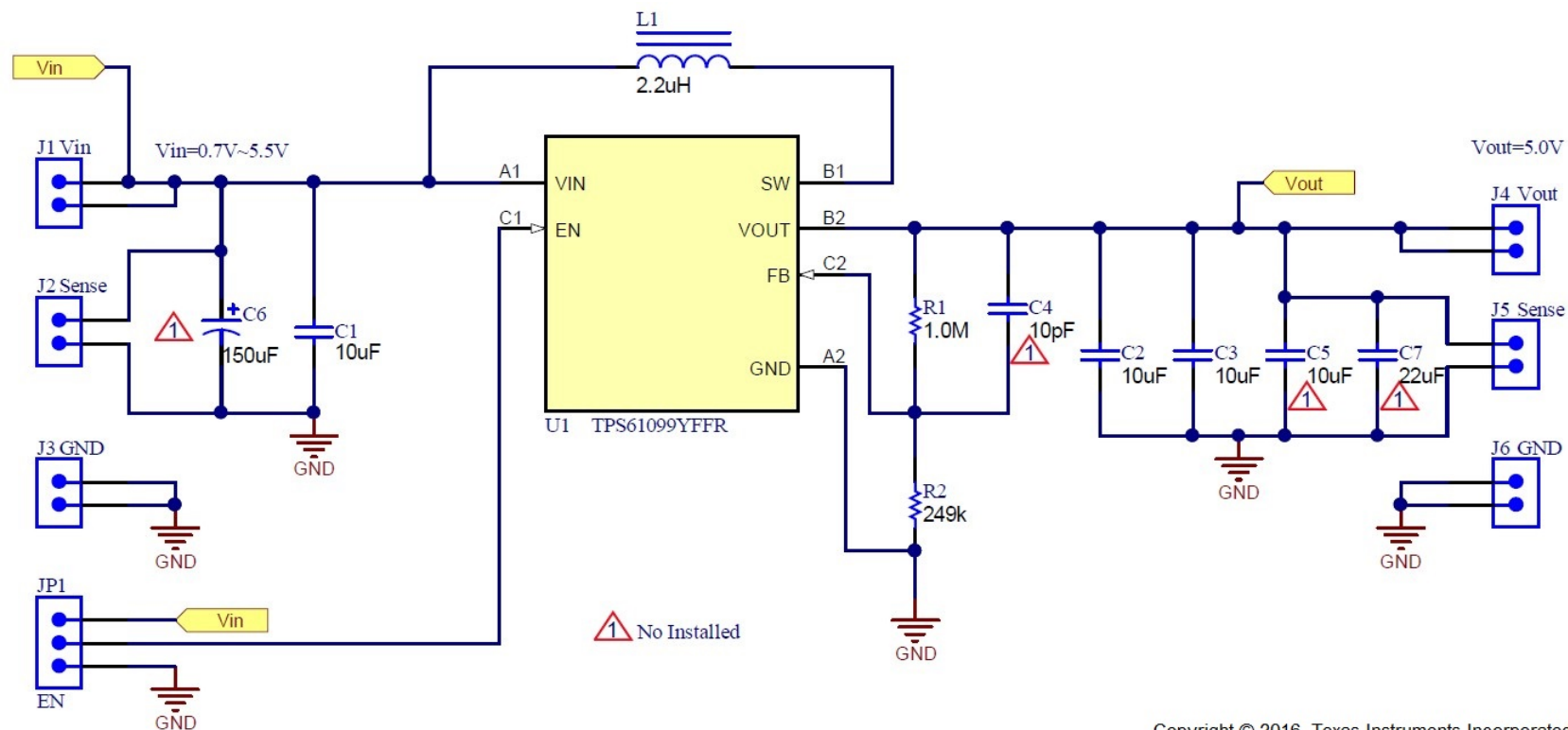
Figure 1. TPS61099 Schematic
