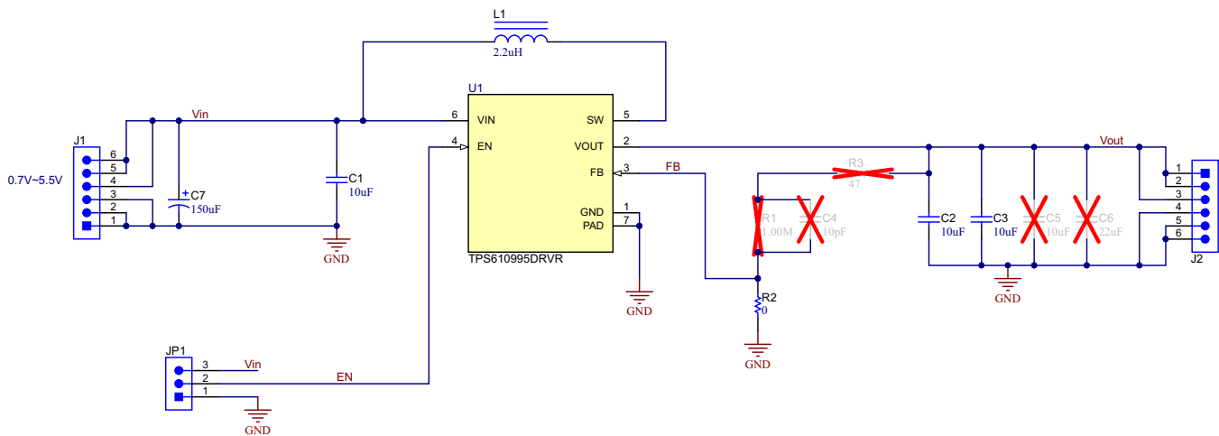
Figure 1. TPS61099EVM-023 Schematic
