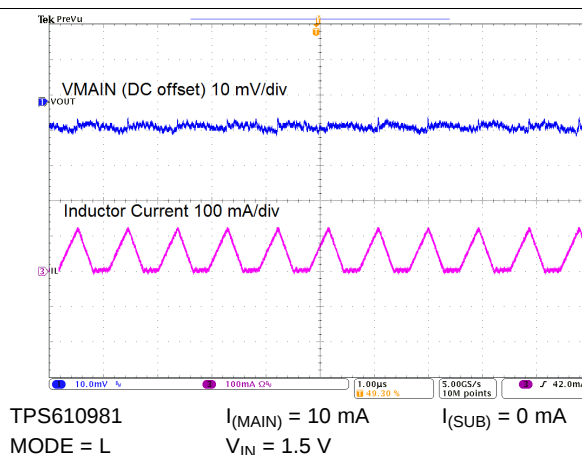
Figure 60. Switching Waveforms
