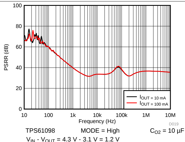
Figure 49. LDO PSRR vs Frequency
