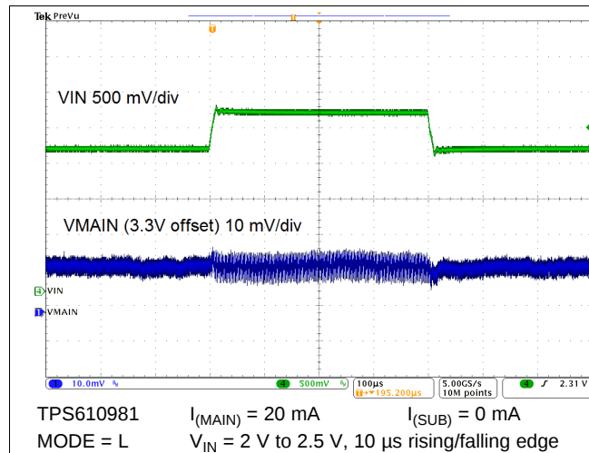
Figure 71. Line Transient Response
