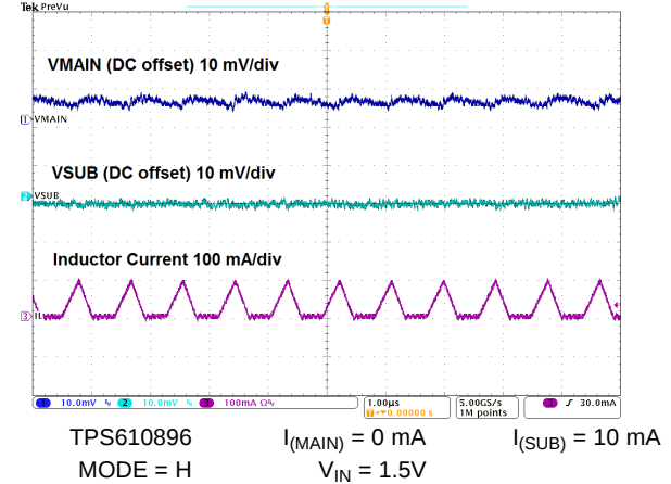
Figure 66. Switching Waveforms
