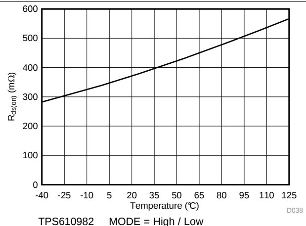
Figure 12. Low Side Switch On Resistance vs Temperature
