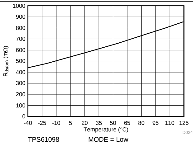
Figure 8. Low Side Switch On Resistance vs Temperature
