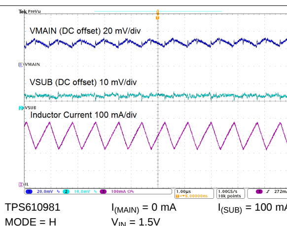
Figure 64. Switching Waveforms
