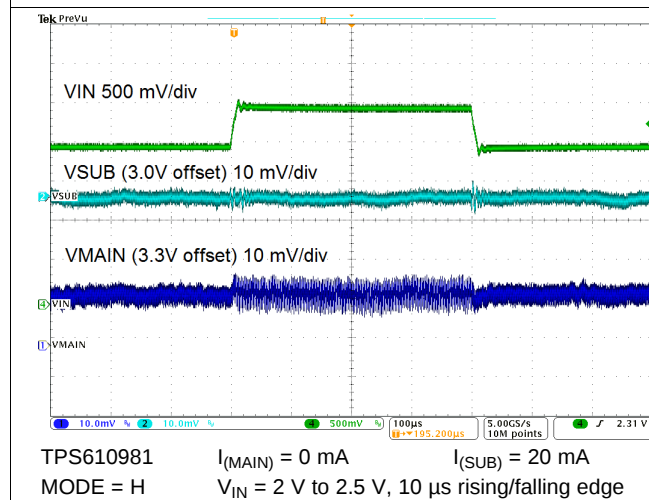
Figure 73. Line Transient Response
