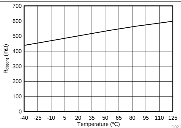
TPS61098 MODE = High
