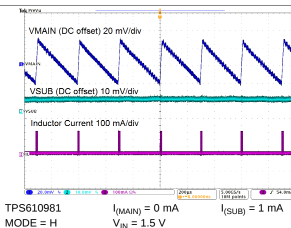
Figure 62. Switching Waveforms
