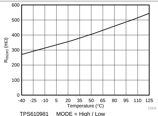
Figure 10. Low Side Switch On Resistance vs Temperature
