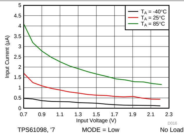
Figure 42. Input Current vs Input Voltage (Low Power Mode)
