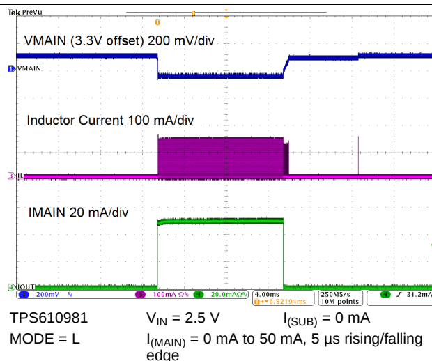
Figure 68. Load Transient Response
