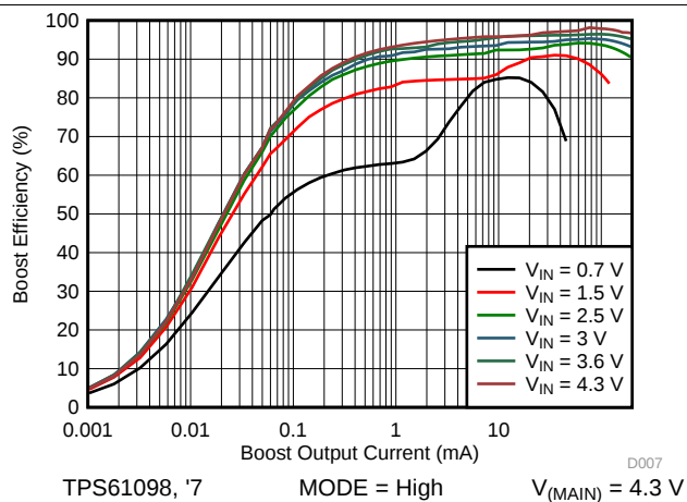
Figure 19. Boost Efficiency vs Output Current (Active Mode)
