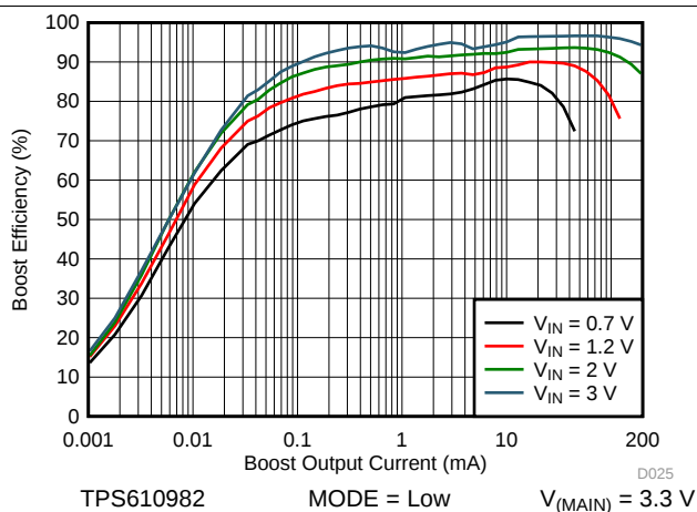
Figure 22. Boost Efficiency vs Output Current (Low Power Mode)
