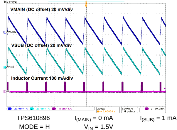
Figure 65. Switching Waveforms
