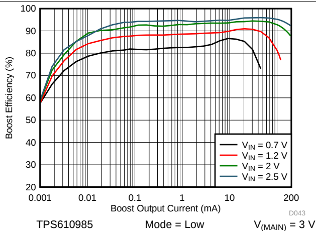
Figure 24. Boost Efficiency vs Output Current (Low Power Mode)
