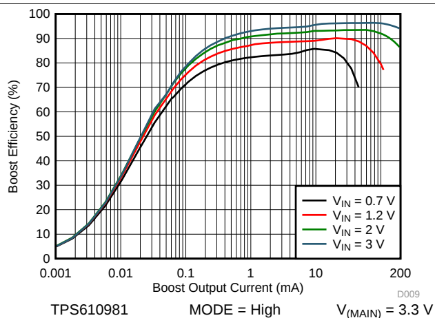
Figure 21. Boost Efficiency vs Output Current (Active Mode)
