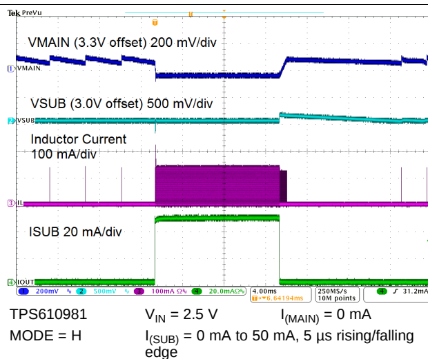
Figure 70. LDO Load Transient Response
