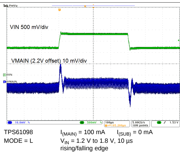
Figure 83. Line Transient Response
