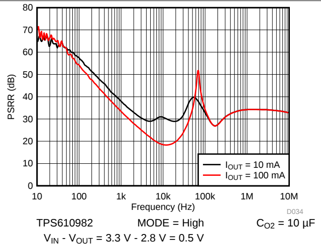
Figure 52. LDO PSRR vs Frequency (Active Mode)
