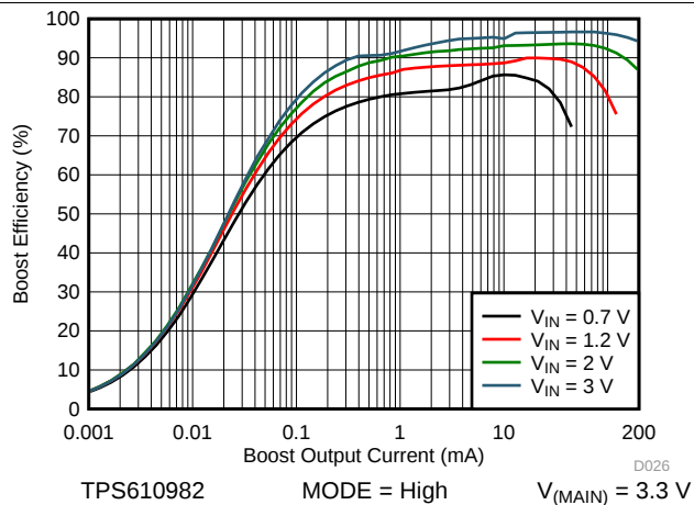
Figure 23. Boost Efficiency vs Output Current (Active Mode)
