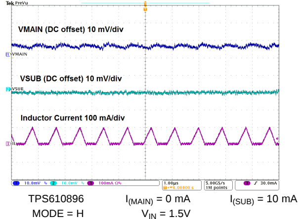
Figure 66. Switching Waveforms
