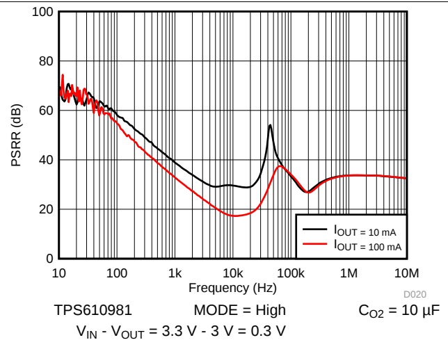
Figure 50. LDO PSRR vs Frequency
