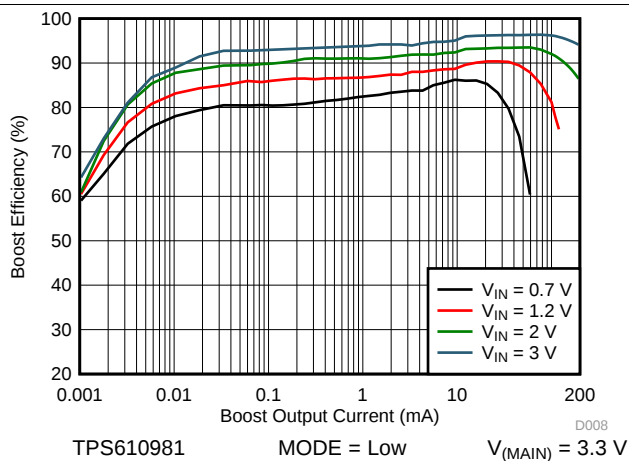
Figure 20. Boost Efficiency vs Output Current (Low Power Mode)
