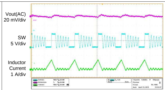
Figure 14. Switching Waveforms in DCM
