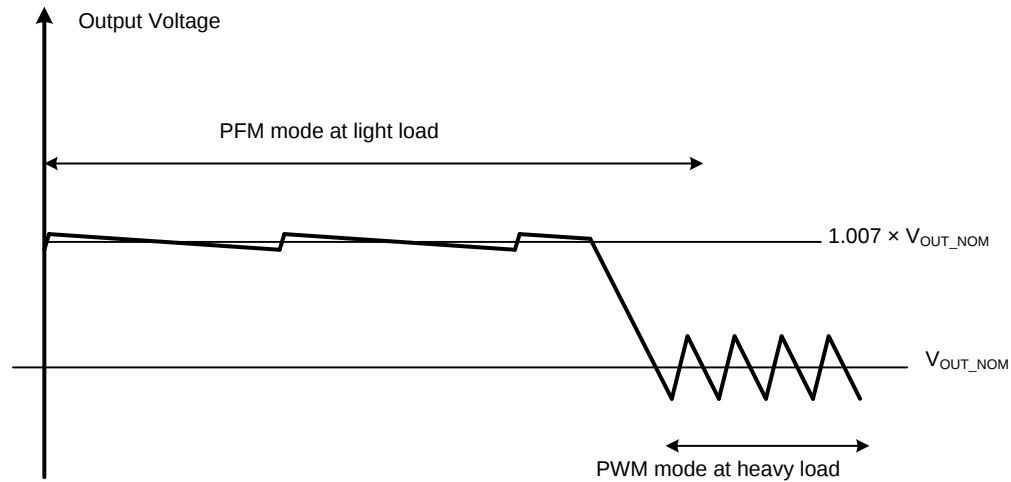
Figure 11. PFM Mode Diagram
