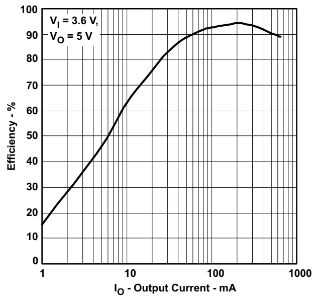
Figure 5. Voltage-Mode Efficiency
