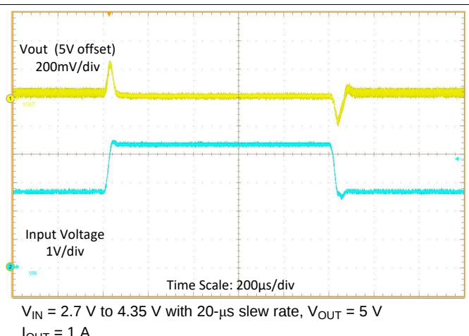
Figure 20. Line Transient
