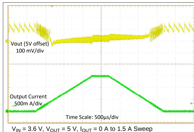
Figure 21. Load Sweep
