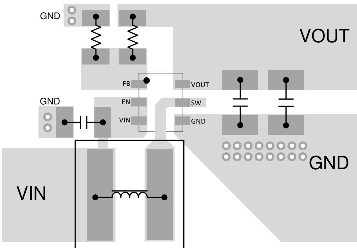
Figure 25. Layout Example
