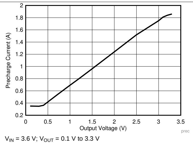
Figure 4. Pre-charge Current vs Output Voltage
