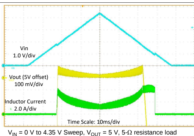
Figure 22. Line Sweep
