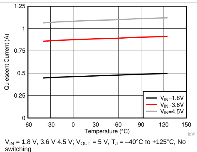
Figure 6. Quiescent Current into VIN vs Temperature
