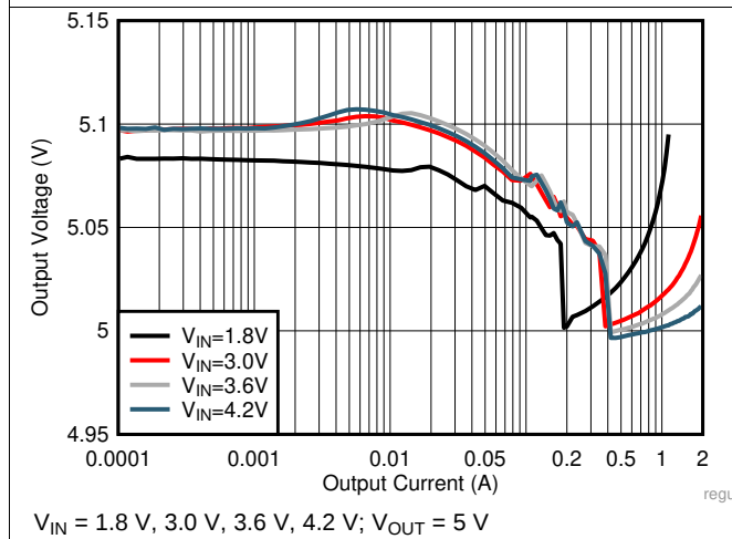
Figure 3. Load Regulation
