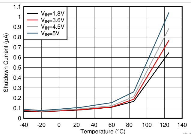
Figure 8. Shutdown Current vs Temperature
