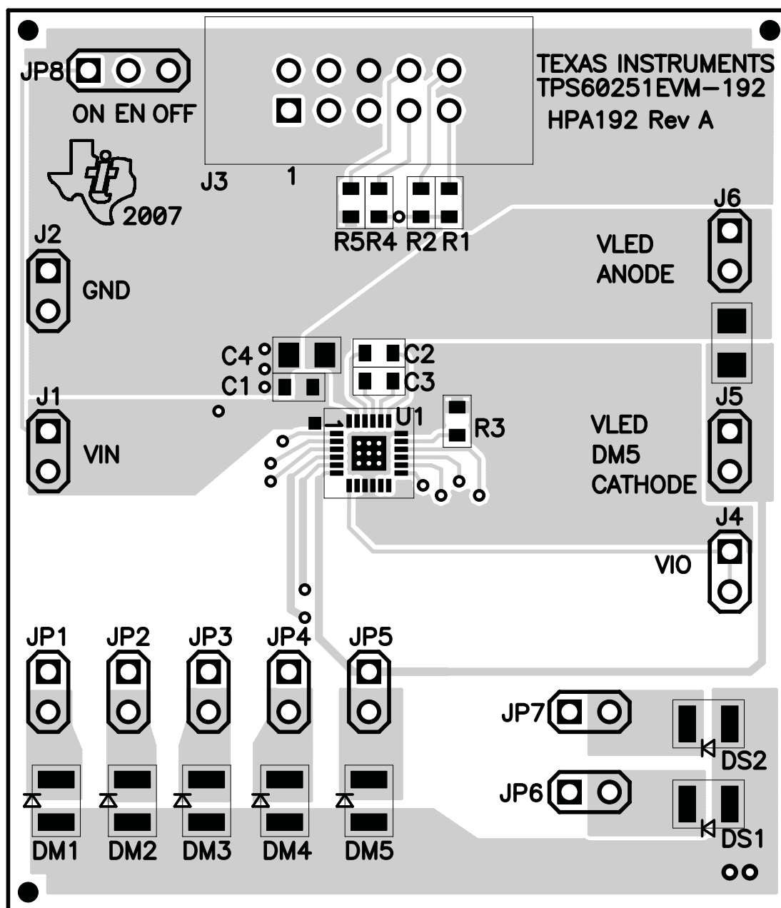
Figure 2. Assembly Layer
