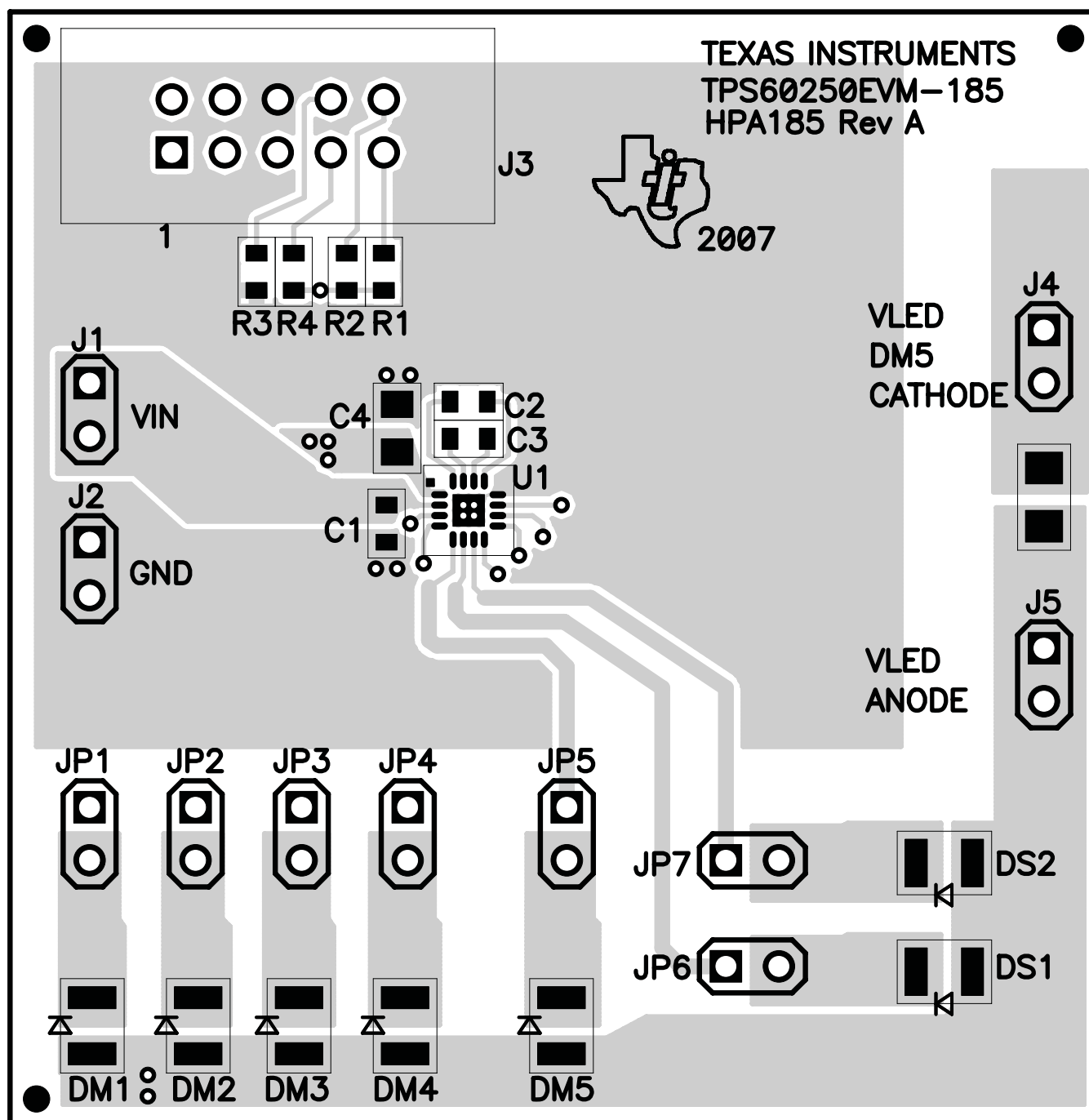
Figure 2. Assembly Layer
