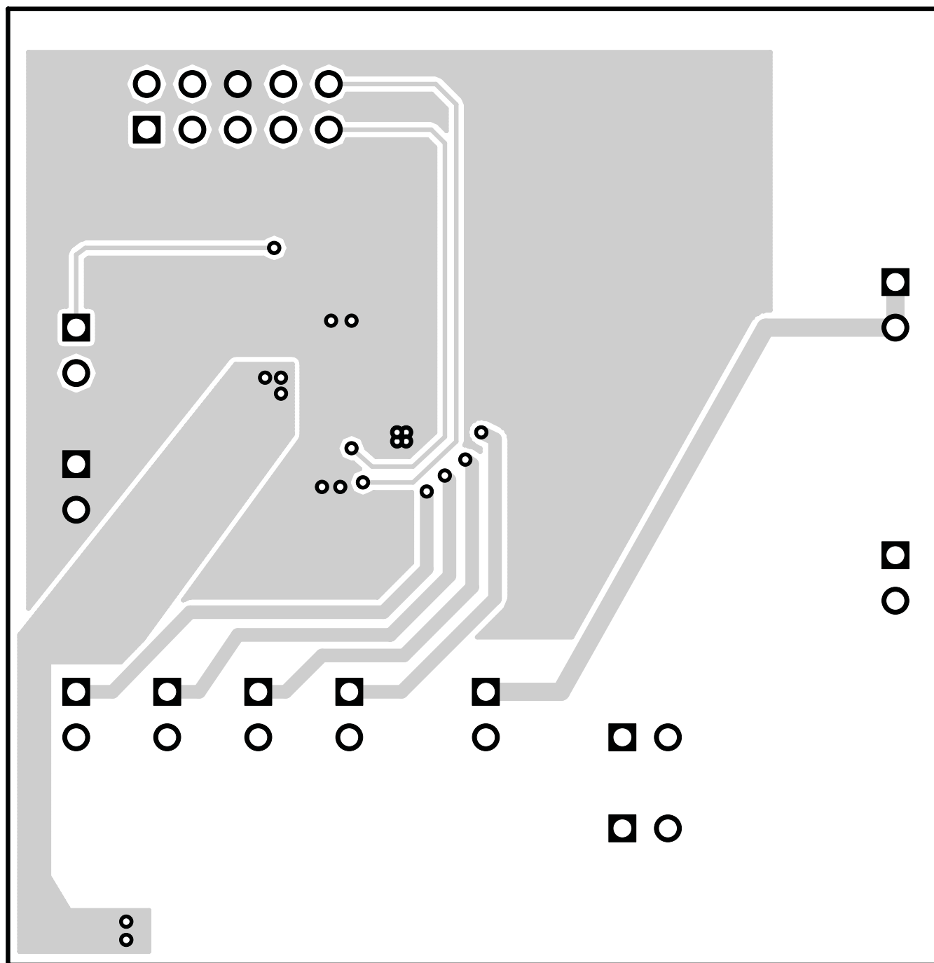
Figure 4. Bottom Layer Routing
