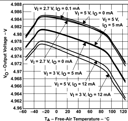
Figure 21. TPS60241
