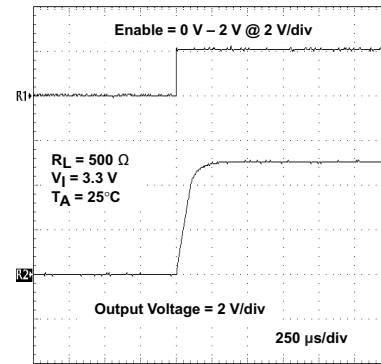
Figure 28. Start-Up Timing
