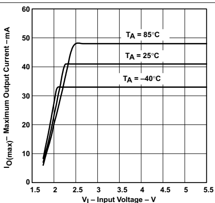
Figure 23. TPS60240
