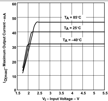
Figure 26. TPS60243
