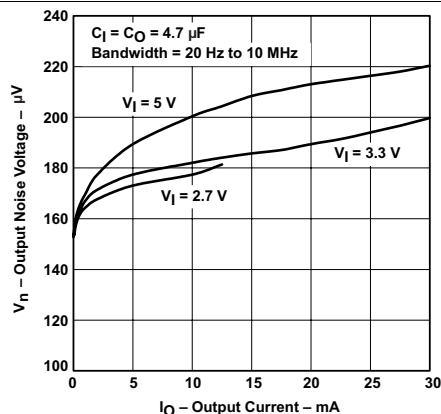
Figure 22. TPS60241
