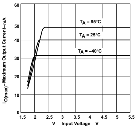
Figure 25. TPS60242
