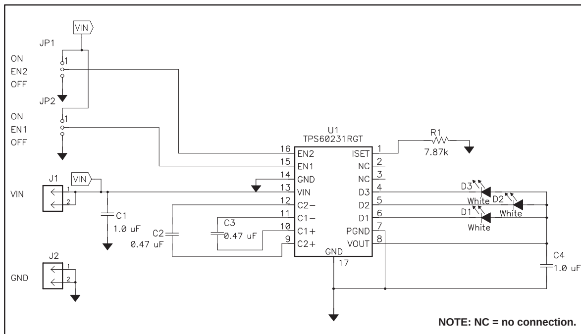
Figure 5. TPS60231EVM-047 Schematic
