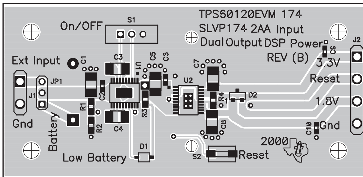
Figure 1–5. Assembly
