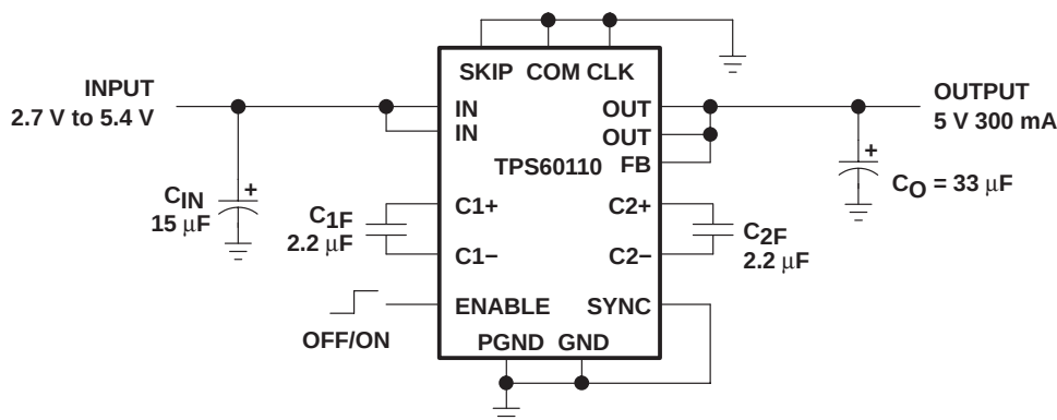
Figure 24. Typical Operating Circuit TPS60110 in Constant Frequency Mode
