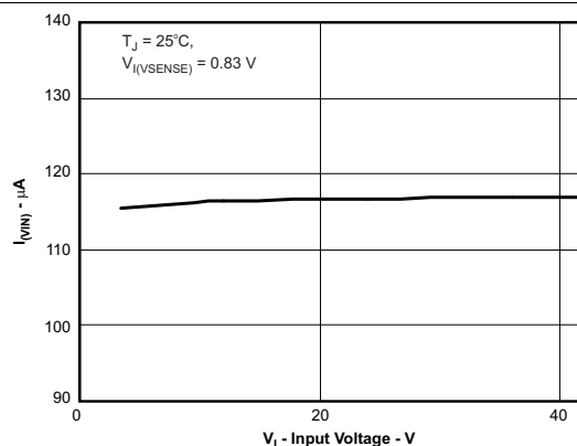
Figure 18. VIN Supply Current vs Input Voltage
