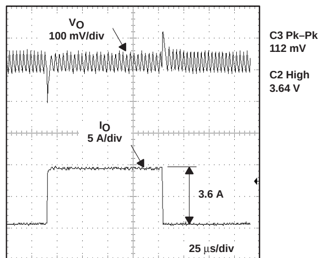
Figure 3–28. SLVP113 Measured Load Transient Waveforms
