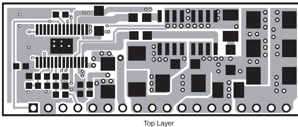
Figure 1–6. Top Layer
