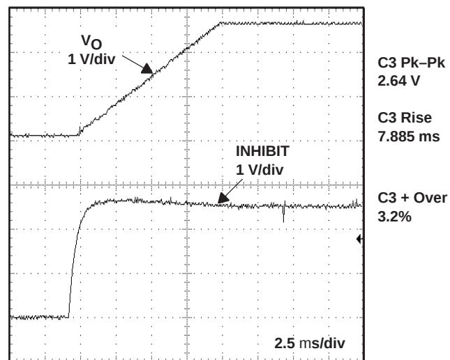
Figure 3–16. SLVP112 Measured Start-Up (INHIBIT) Waveforms
