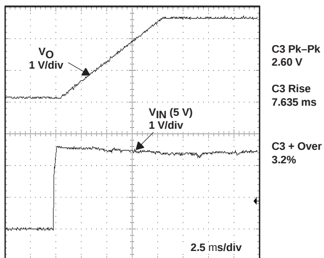
Figure 3–18. SLVP112 Measured Start-Up ( V_{IN} ) Waveforms
