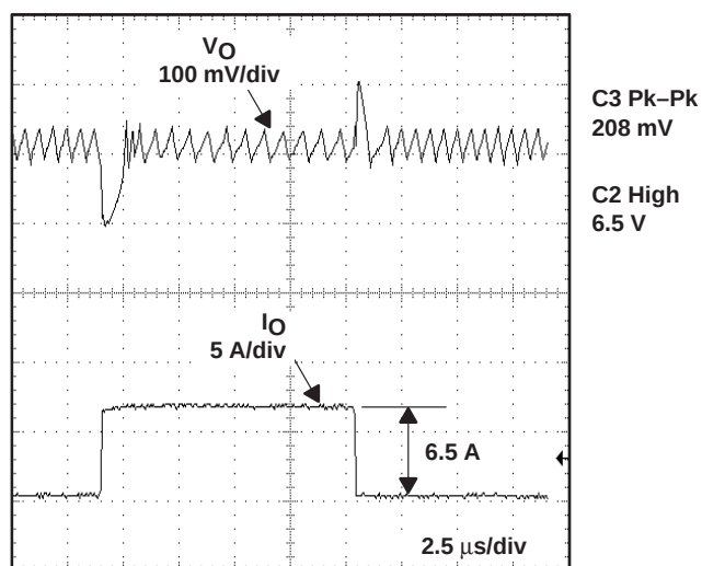
Figure 3–11. SLVP112 Measured Load Regulation
