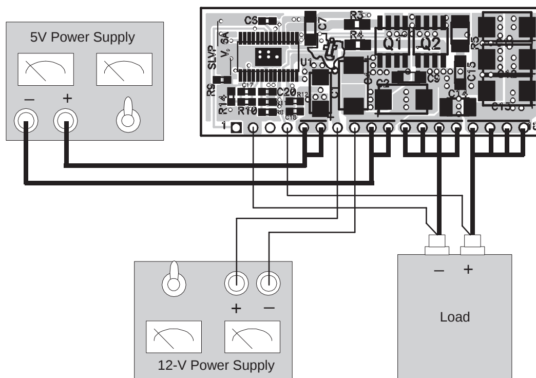
Figure 3–1. Test Setup
