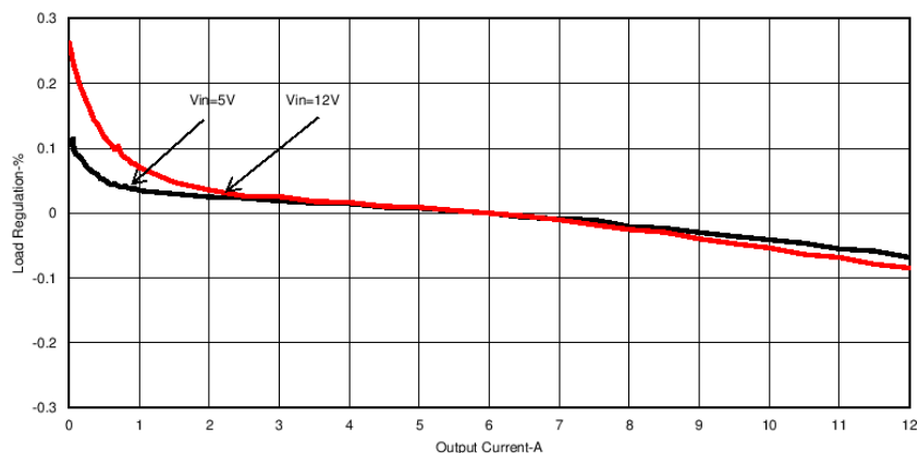
Figure 7. TPS56C20EVM-614 Load Regulation
