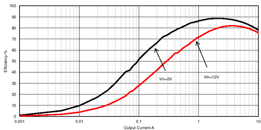
Figure 6. TPS56C20EVM-614 Efficiency (Low Current)
