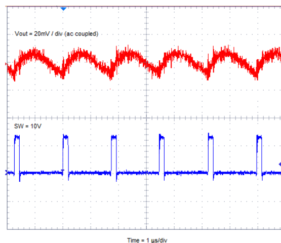
Figure 10. TPS56C20EVM-614 Output Voltage Ripple
