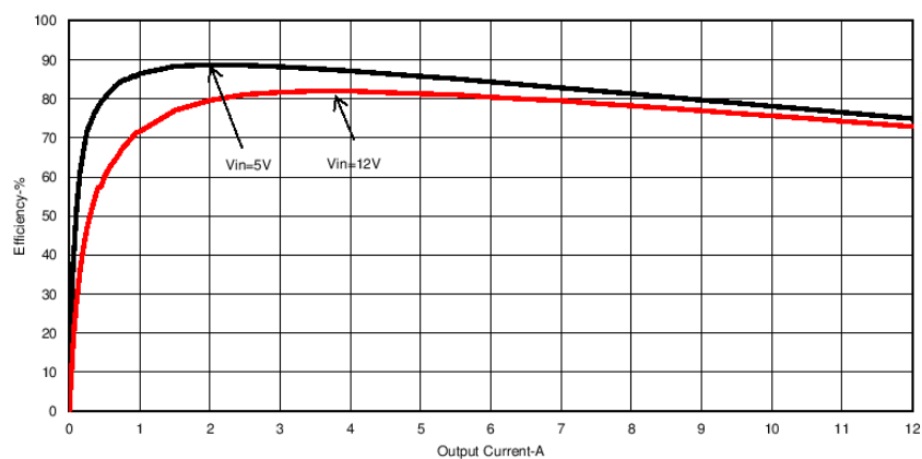
Figure 5. TPS56C20EVM-614 Efficiency
