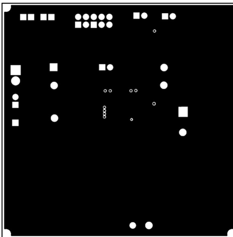
Figure 18. Internal Layer 2
