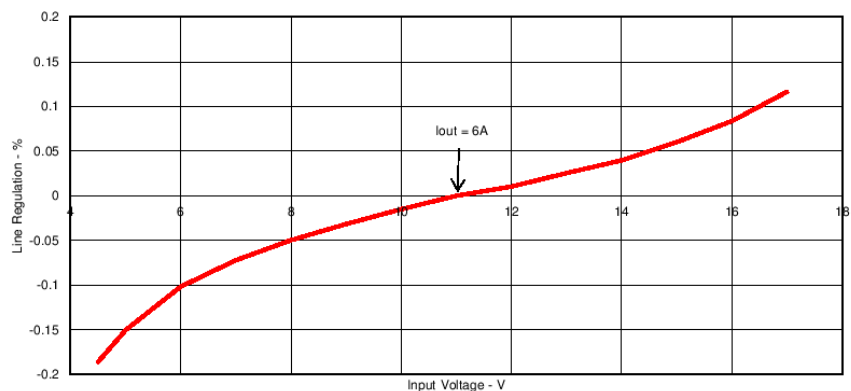
Figure 8. TPS56C20EVM-614 Line Regulation
