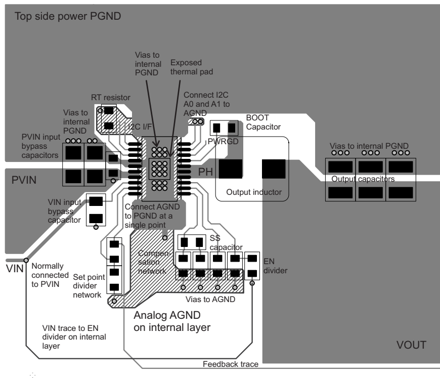
Figure 39. PCB Layout
