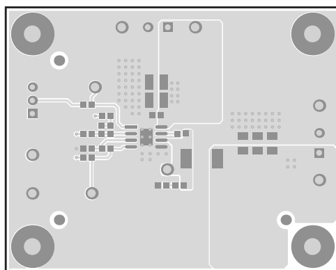
Figure 15. Top Layer
