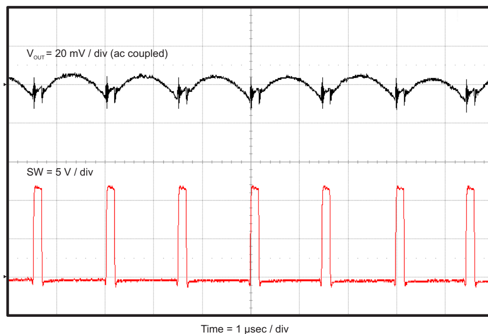
Figure 6. TPS56628EVM-534 Output Voltage Ripple ( I_{OUT} = 6 A)
