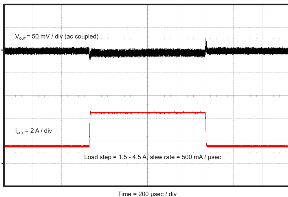
Figure 5. TPS56628EVM-534 Load Transient Response
