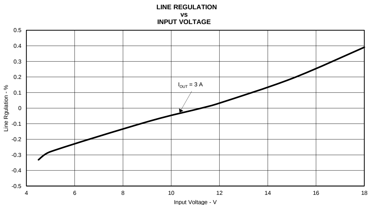
Figure 4. TPS56628EVM-534 Line Regulation
