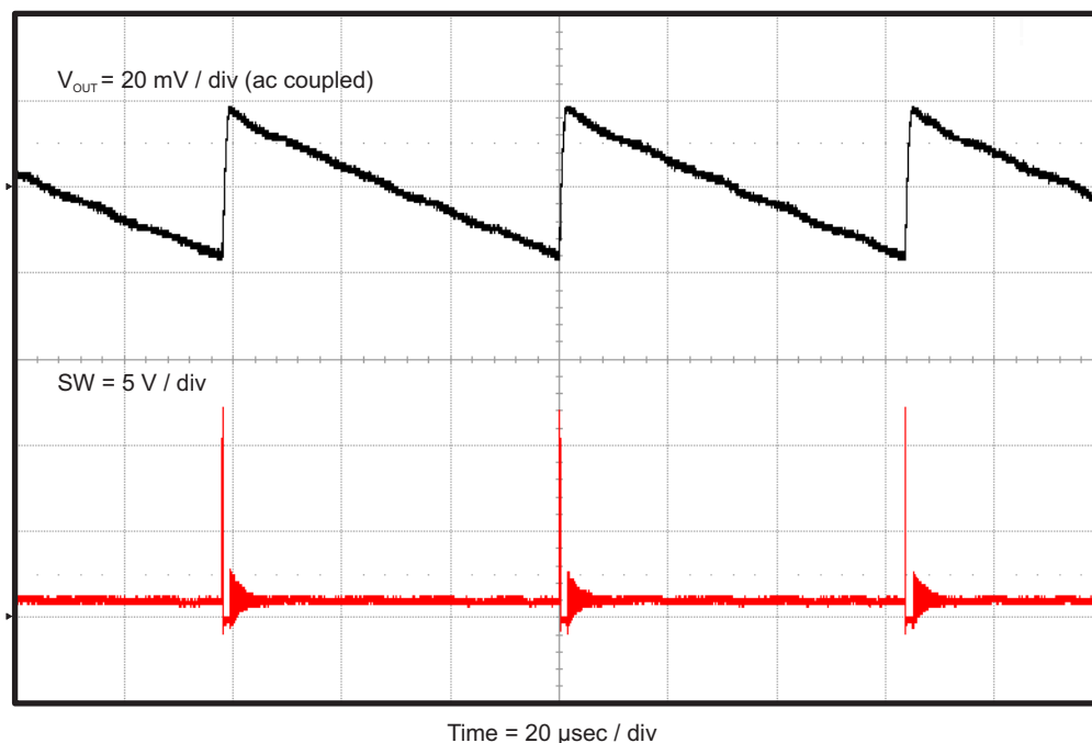
Figure 8. TPS56628EVM-534 Output Voltage Ripple ( I_{OUT} = 10 mA)
