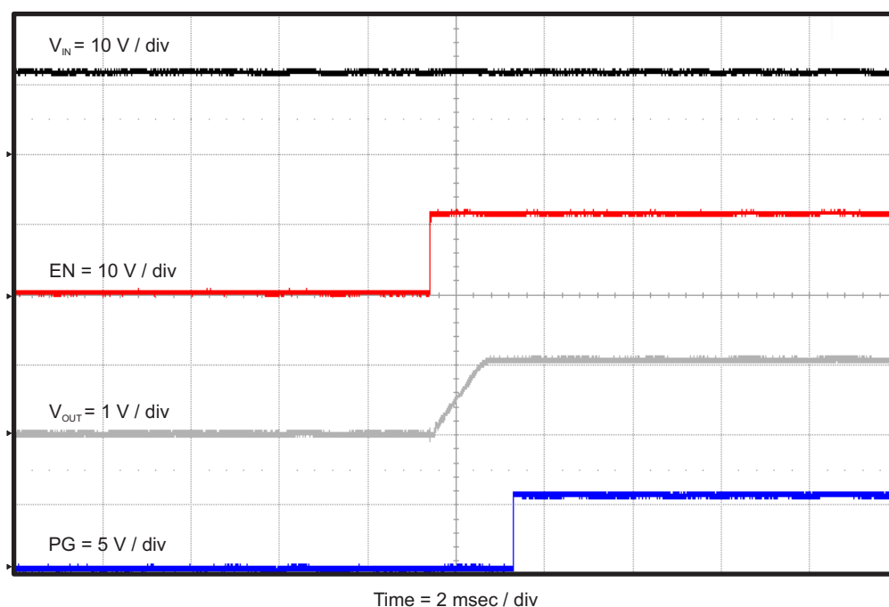
Figure 11. TPS56628EVM-534 Start-Up Relative to EN With VREG5, PG and V_{OUT}
