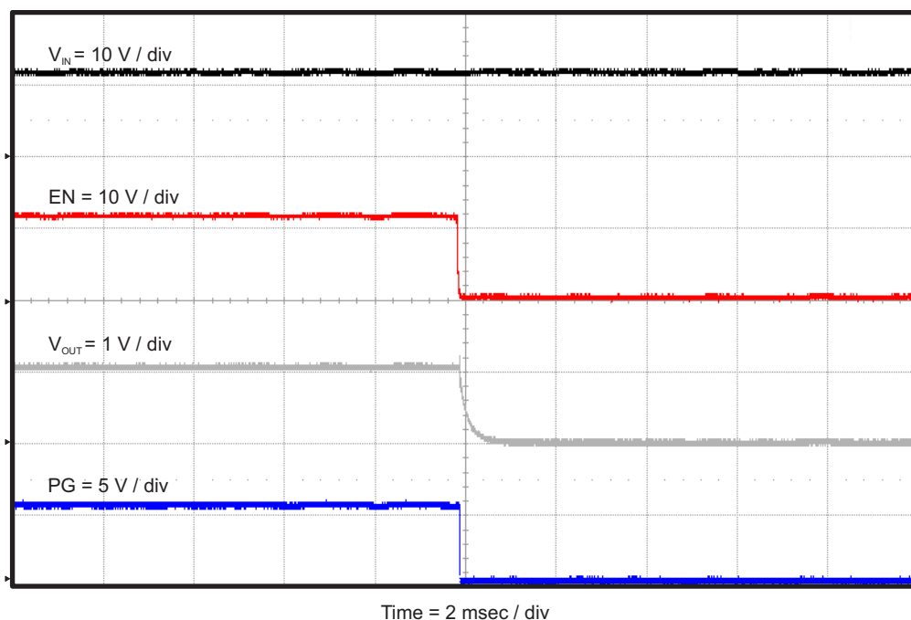
Figure 13. TPS56628EVM-534 Shut-Down Relative to EN With VREG5, PG and V_{OUT}
