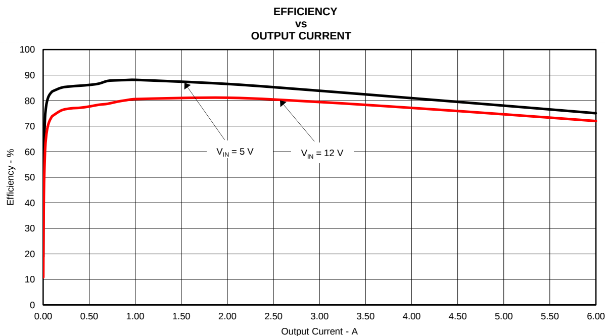
Figure 1. TPS56628EVM-534 Efficiency
