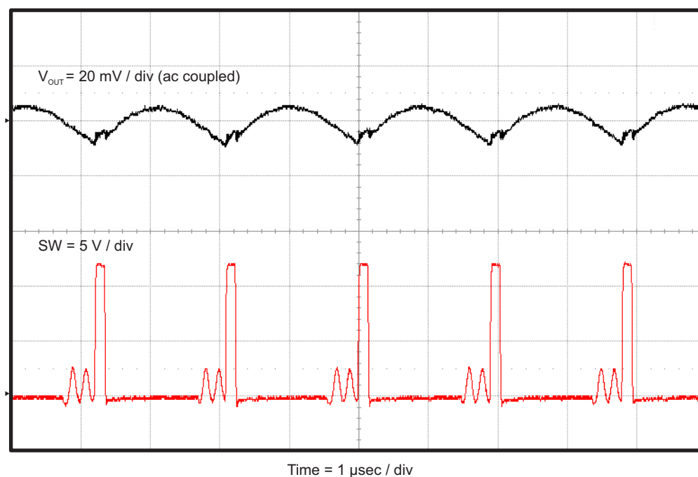
Figure 7. TPS56628EVM-534 Output Voltage Ripple ( I_{OUT} = 500 mA)
