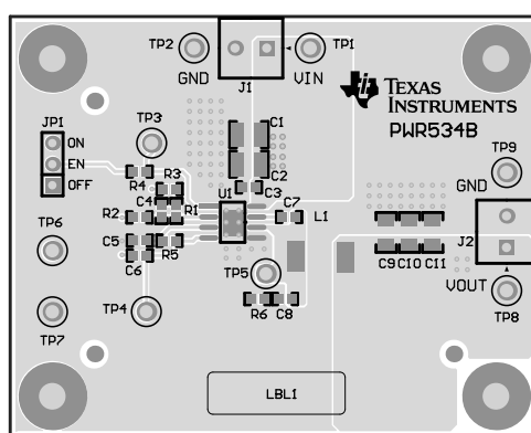
Figure 14. Top Assembly
