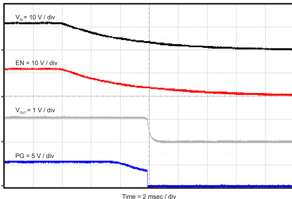
Figure 12. TPS56628EVM-534 Shut-Down Relative to V_{IN} With VREG5, PG and V_{OUT}
