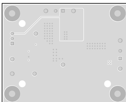
Figure 17. Internal Layer 2
