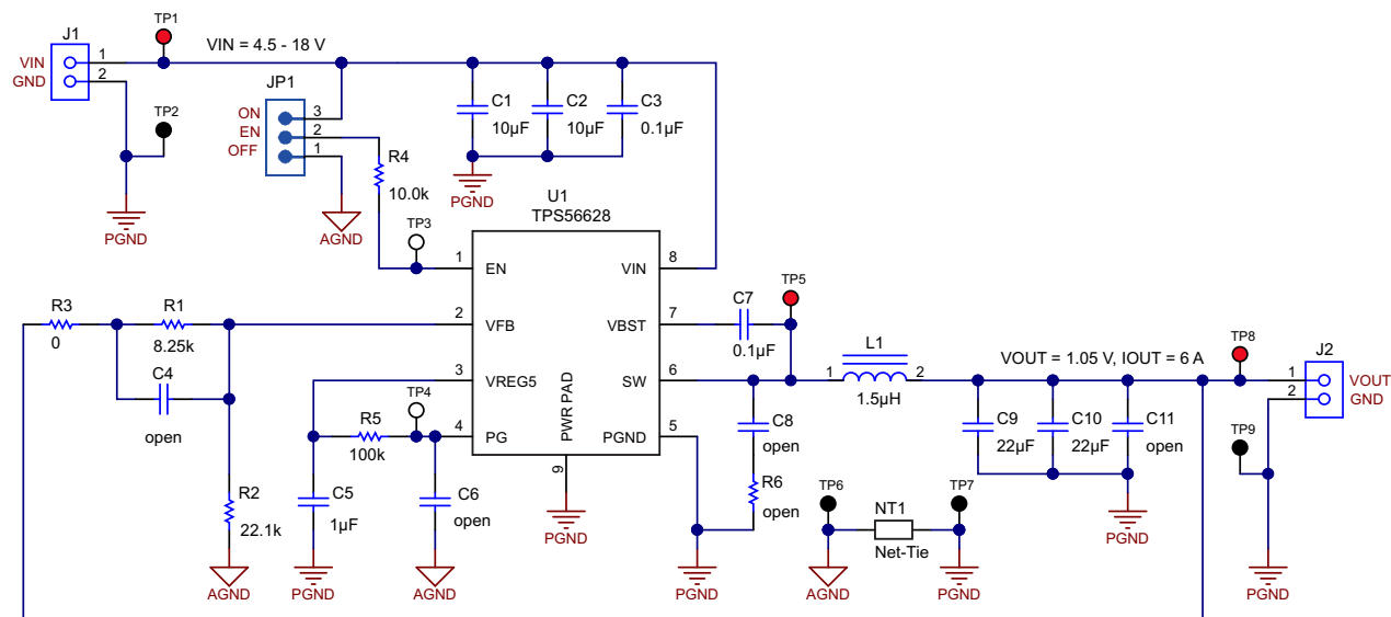
Figure 19. TPS56628EVM-534 Schematic Diagram
