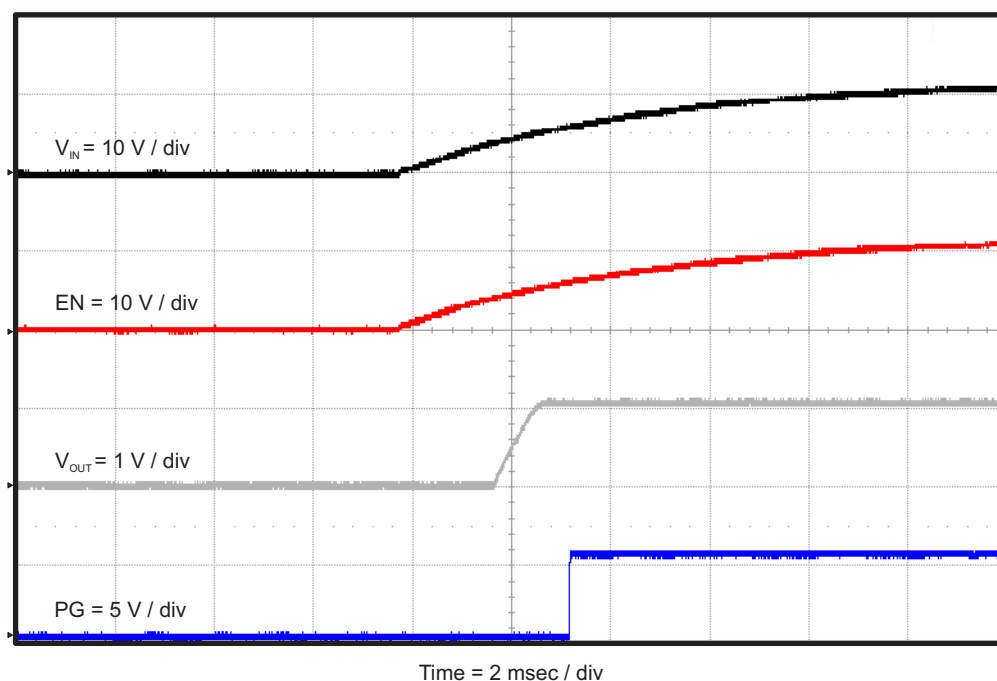
Figure 10. TPS56628EVM-534 Start-Up Relative to V_{IN} With VREG5, PG and V_{OUT}
