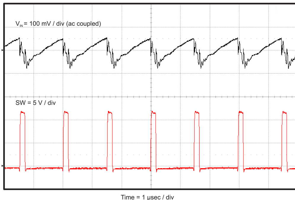
Figure 9. TPS56628EVM-534 Input Voltage Ripple
