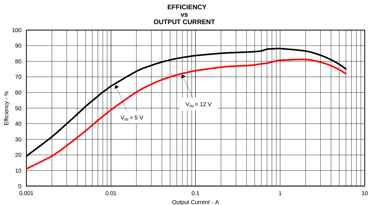
Figure 2. TPS56628EVM-534 Light-Load Efficiency
