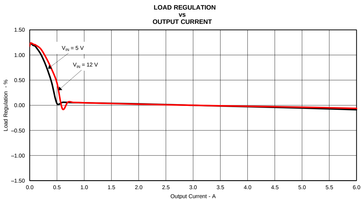
Figure 3. TPS56628EVM-534 Load Regulation, V_{IN} = 5\text{ V} and V_{IN} = 12\text{ V}
