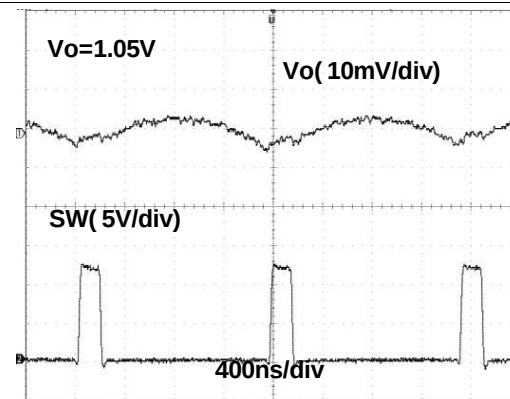
Figure 16. VOUT Ripple
