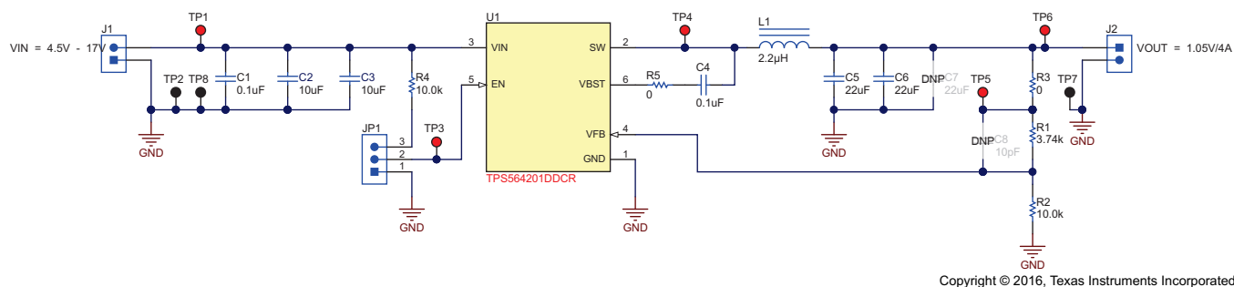
Figure 17. TPS564201EVM-801 Schematic Diagram
