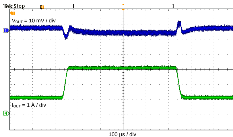
Figure 5. Load Transient Response, 1 A to 3 A
