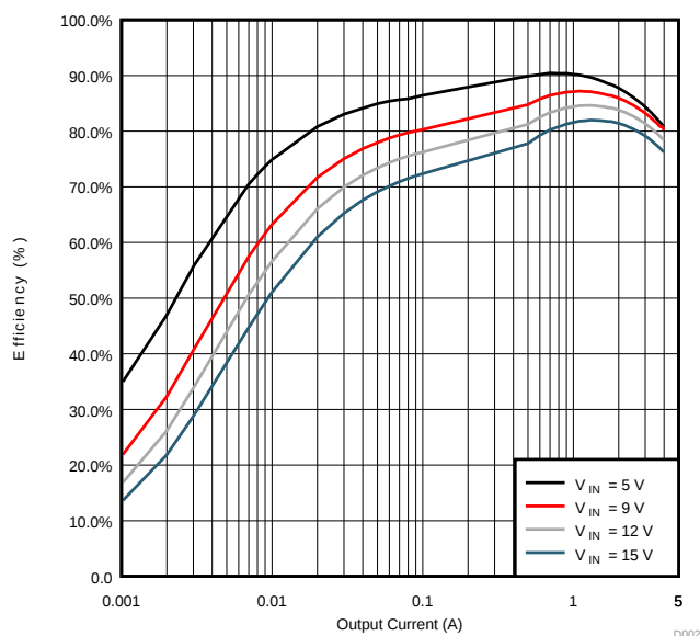
Figure 2. Light Load Efficiency
