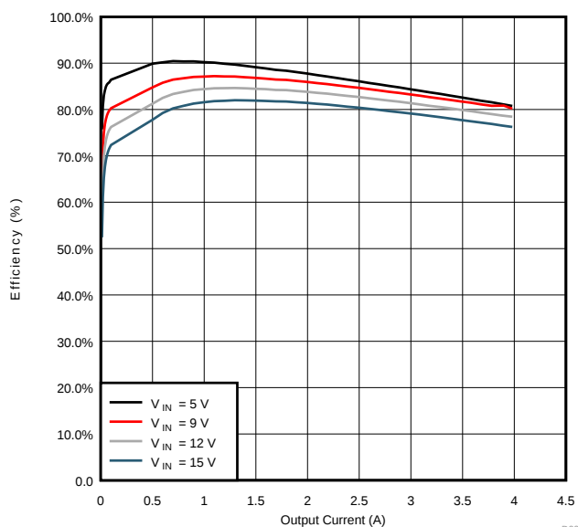
Figure 1. Efficiency
