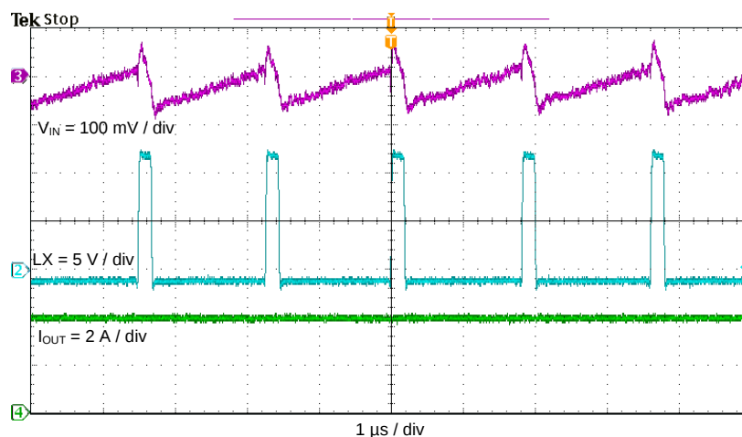
Figure 9. Input Voltage Ripple
