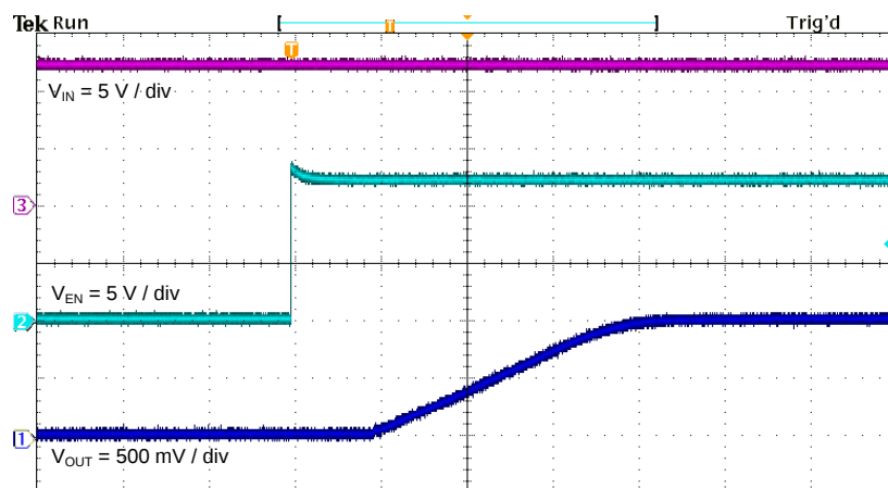
Figure 11. Start-Up Relative to EN
