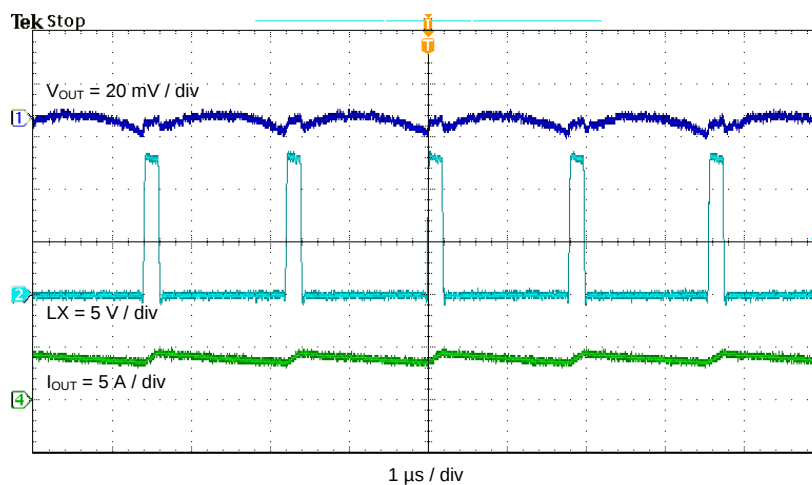
Figure 6. Output Voltage Ripple, I_{OUT} = 4 A
