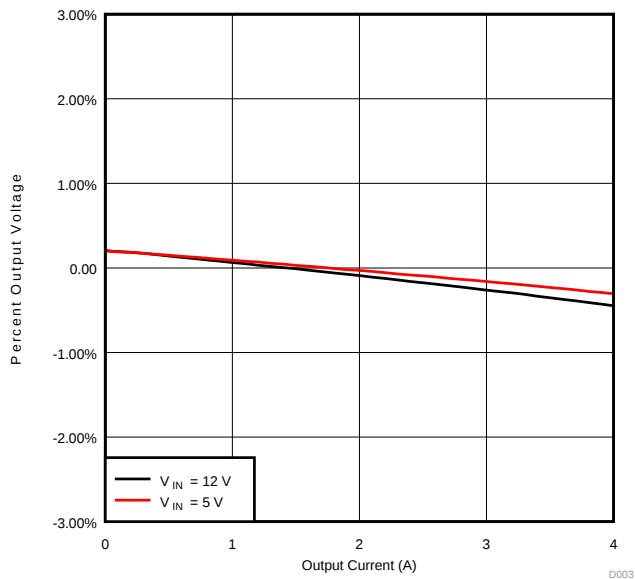
Figure 3. Load Regulation
