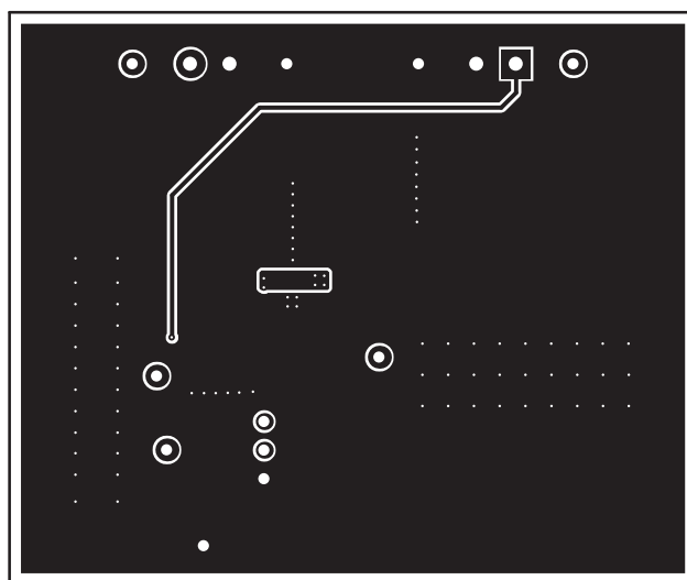
Figure 16. Bottom Layer
