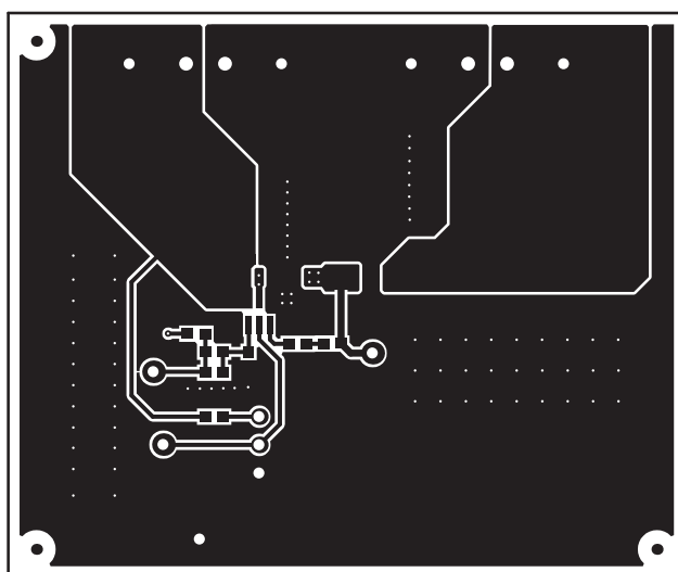
Figure 15. Top Layer
