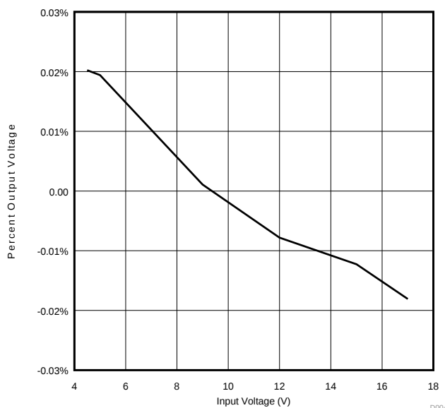
Figure 4. Line Regulation
