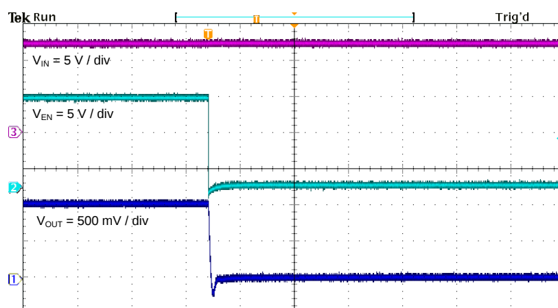
Figure 13. Shut-Down Relative to EN
