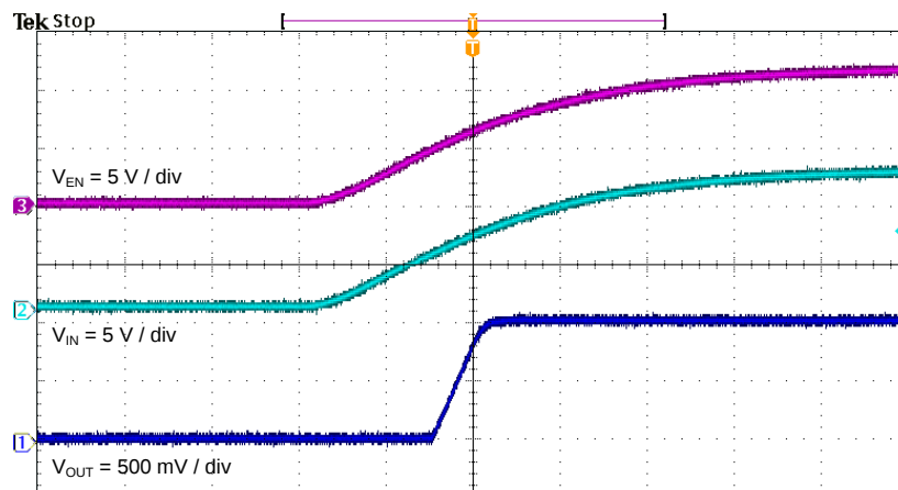
Figure 10. Start-Up Relative to V_{IN}
