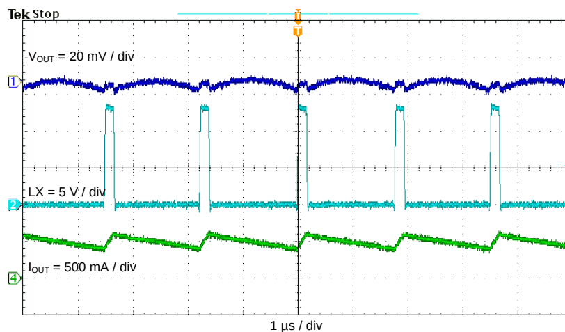
Figure 7. Output Voltage Ripple, I_{OUT} = 2 A
