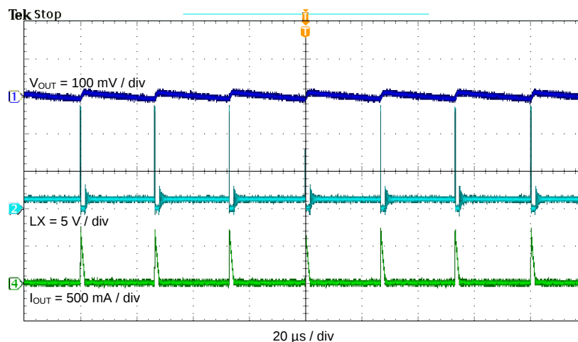
Figure 8. TPS564201 Output Voltage Ripple, no Load
