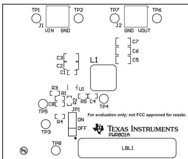
Figure 14. Top Assembly
