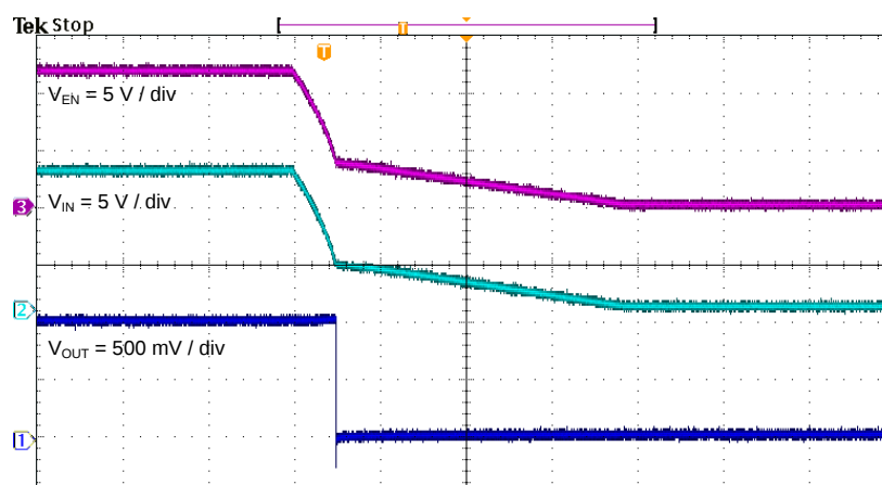
Figure 12. Shut-Down Relative to V_{IN}
