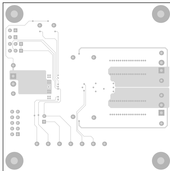
Figure 30. TPS563900EVM-574 Internal Layer-2 Layout
