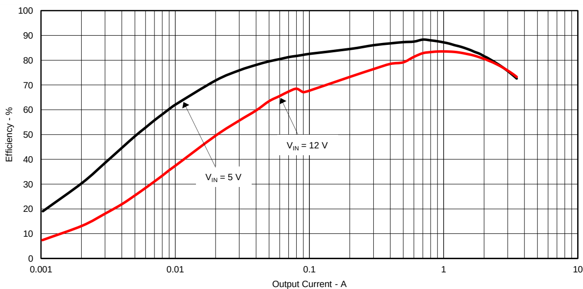
Figure 9. TPS563900EVM-574 V OUT2 SKIP Mode Low Current Efficiency
