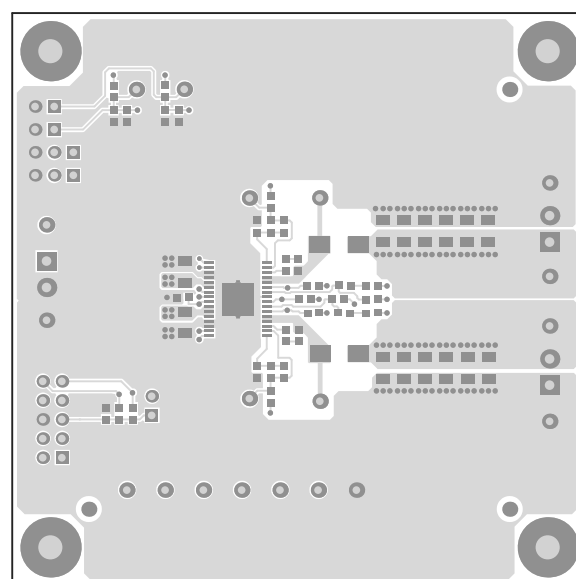
Figure 28. TPS563900EVM-574 Top-Side Layout
