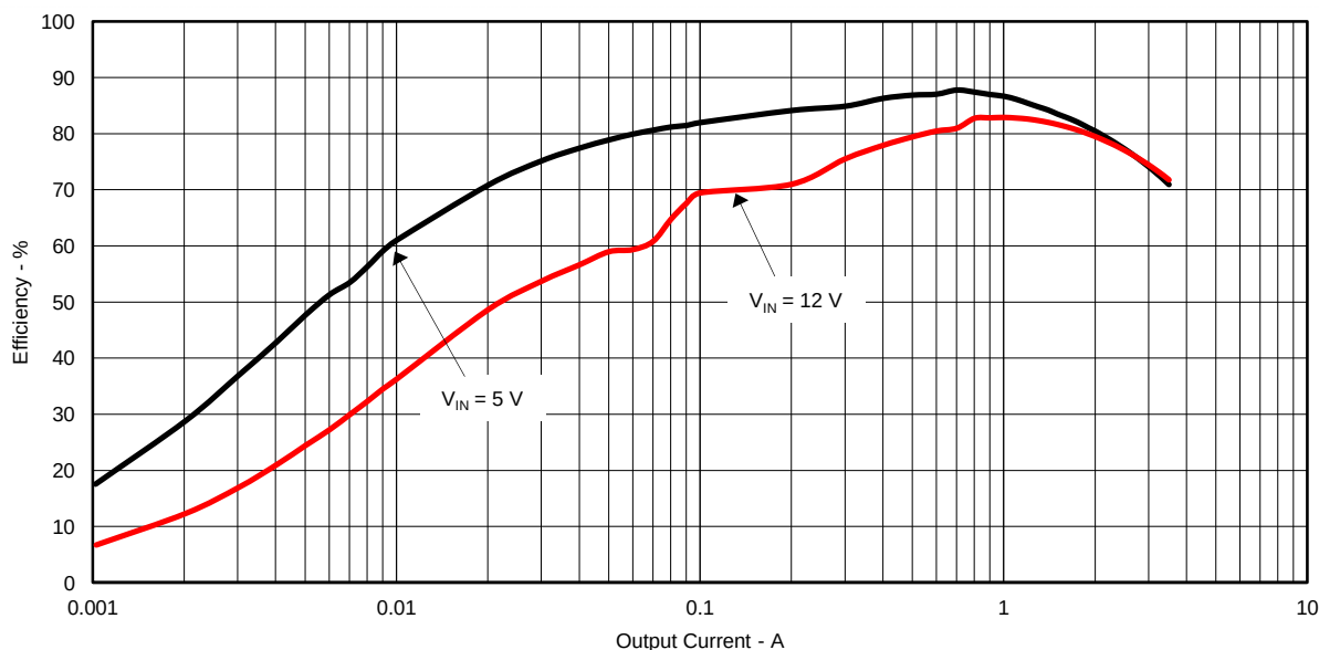
Figure 8. TPS563900EVM-574 V OUT1 SKIP Mode Low Current Efficiency
