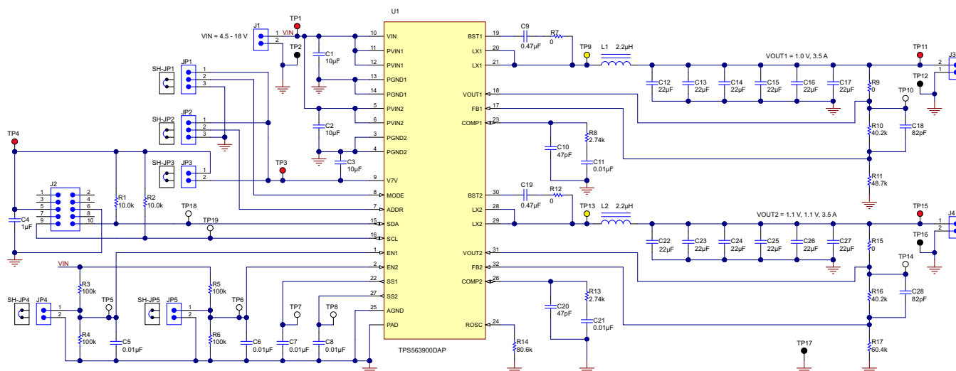
Figure 32. TPS563900EVM-574 Schematic
