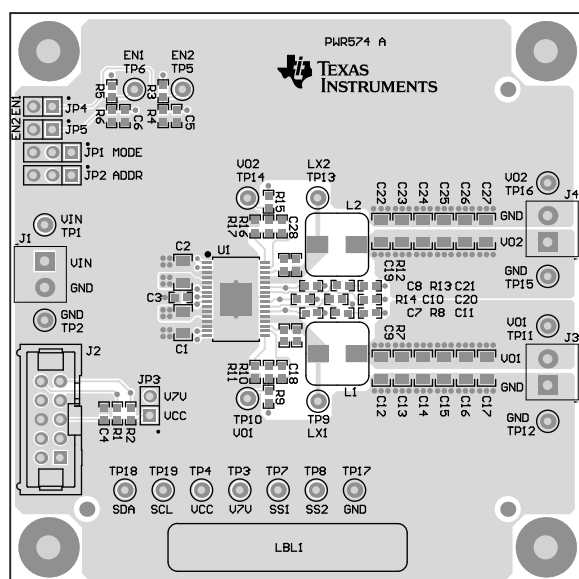
Figure 27. TPS563900EVM-574 Top-Side Assembly
