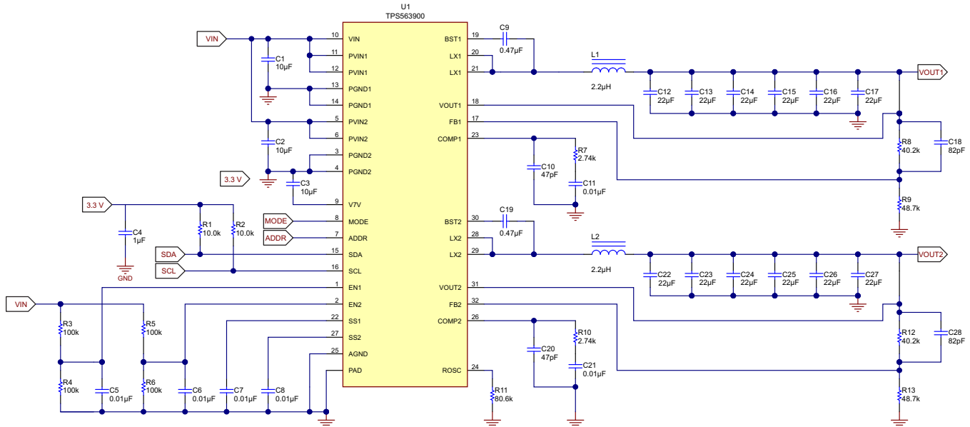
Figure 31. 1.1-V Output TPS563900 Design Example
