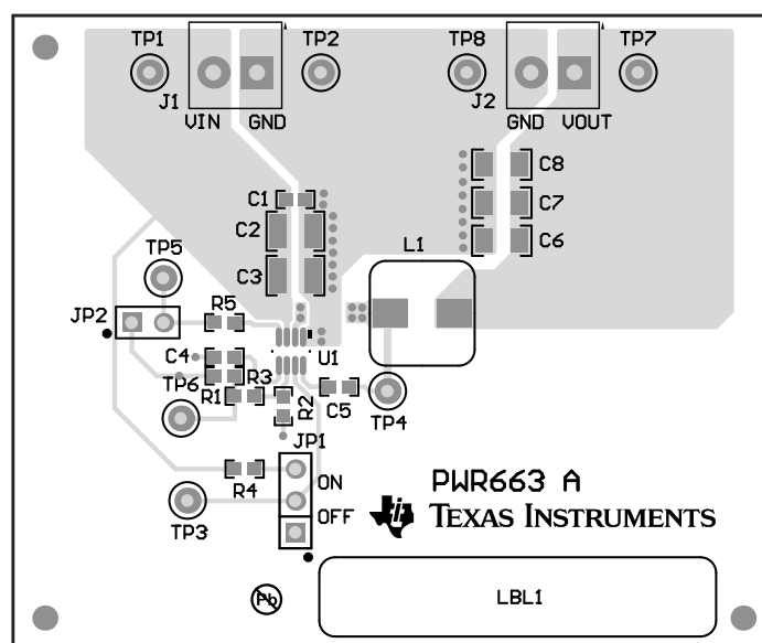
Figure 13. Top Assembly
