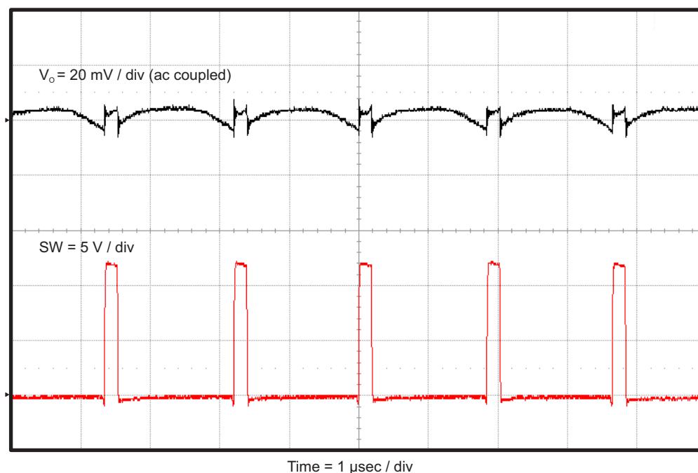
Figure 7. TPS563210AEVM-663 Output Voltage Ripple, I_{OUT} = 3 \text{ A}
