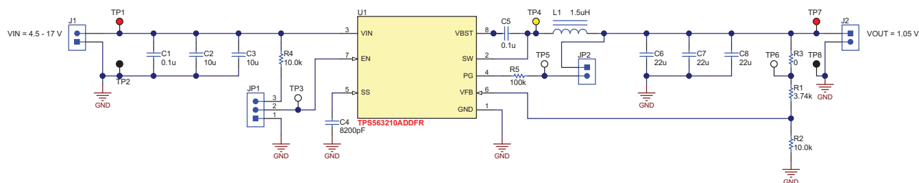
Figure 18. TPS563210AEVM-663 Schematic Diagram
