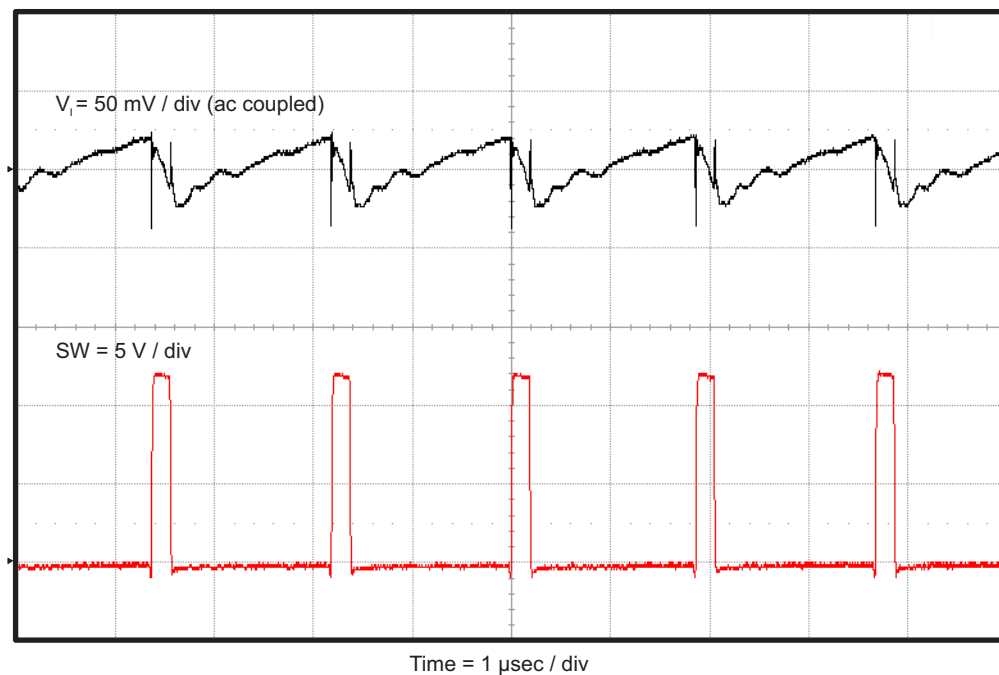
Figure 10. TPS563210AEVM-663 Input Voltage Ripple, I_{OUT} = 3 A
