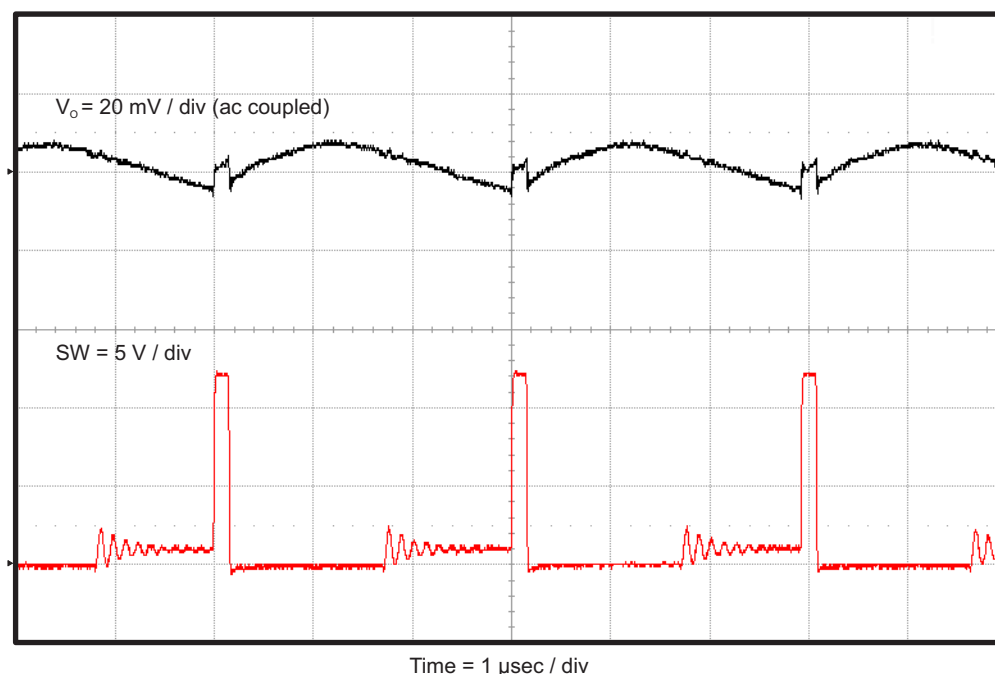
Figure 8. TPS563210AEVM-663 Output Voltage Ripple, I_{OUT} = 300 \text{ mA}
