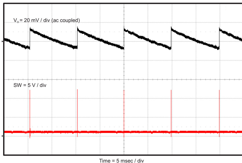
Figure 9. TPS563210AEVM-663 Output Voltage Ripple, I_{OUT} = 0 mA
