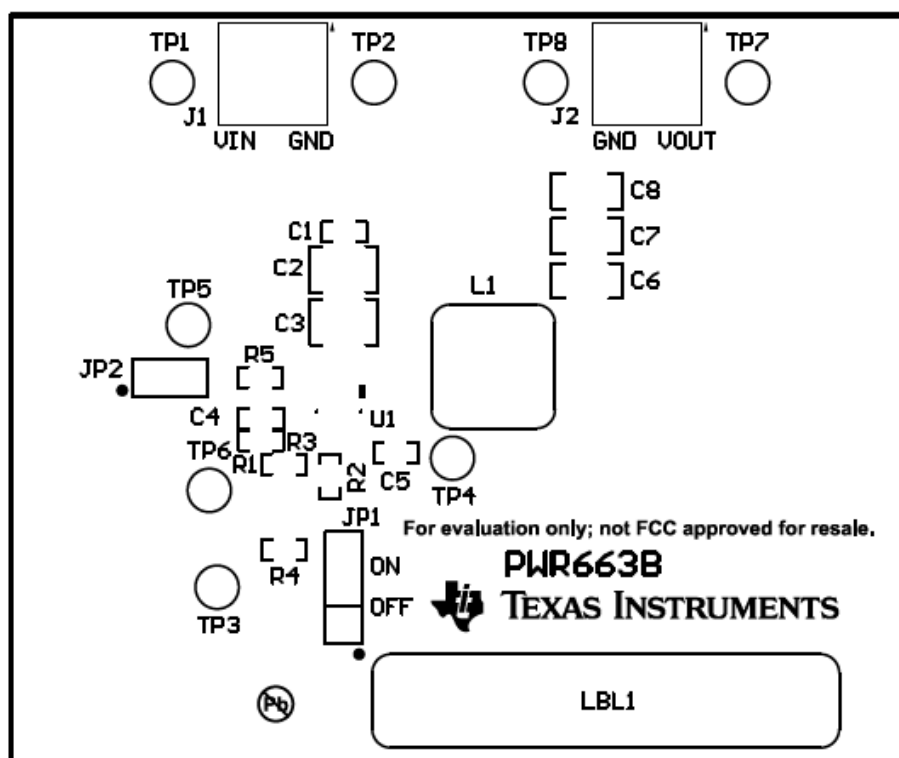
Figure 15. Top Assembly
