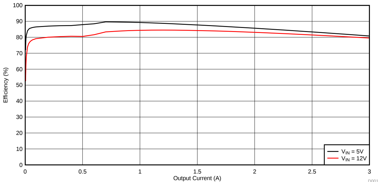
Figure 1. TPS563210AEVM-663 Efficiency
