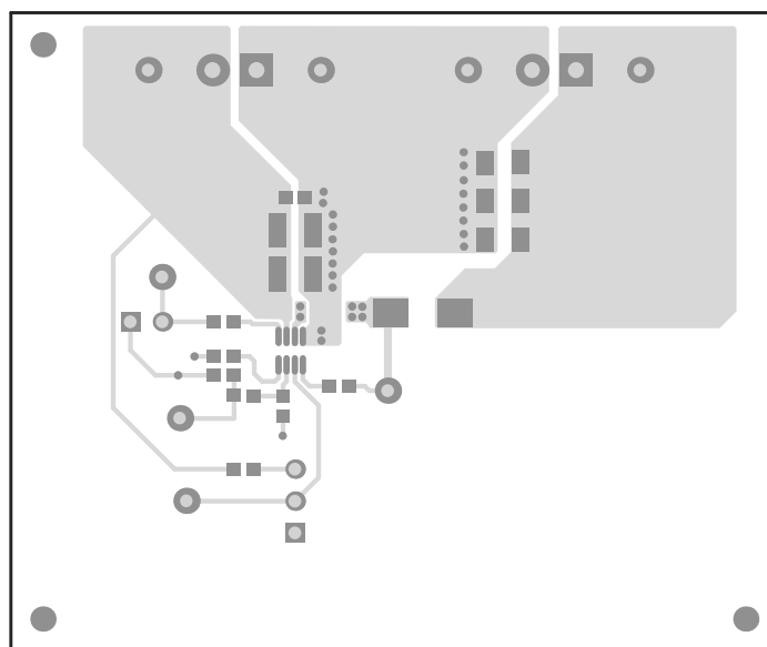
Figure 14. Top Layer
