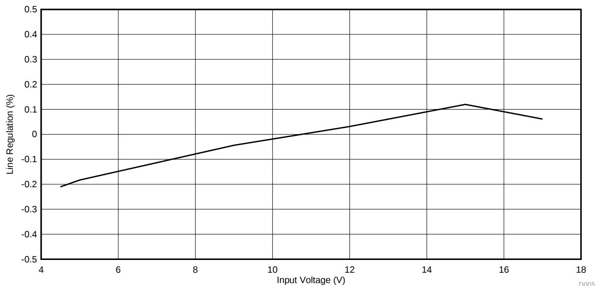
Figure 5. TPS562219EVM-663 Line Regulation
