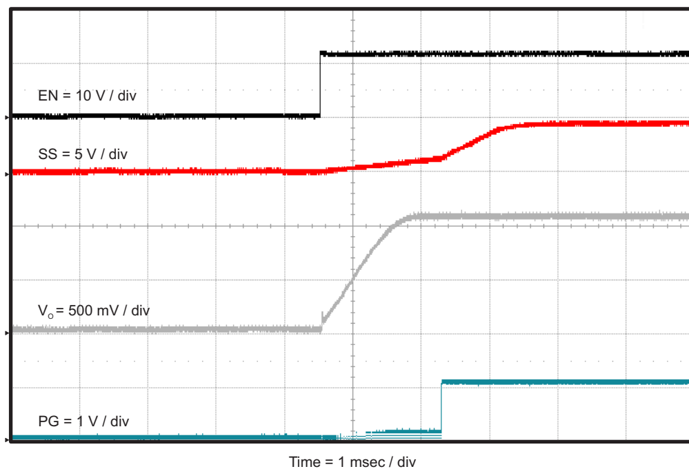
Figure 10. TPS562219EVM-663 Start-Up Relative to EN
