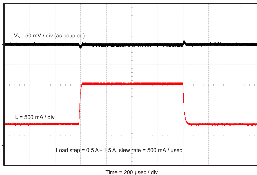
Figure 6. TPS562219EVM-663 Load Transient Response, 25% to 75% Load Step
