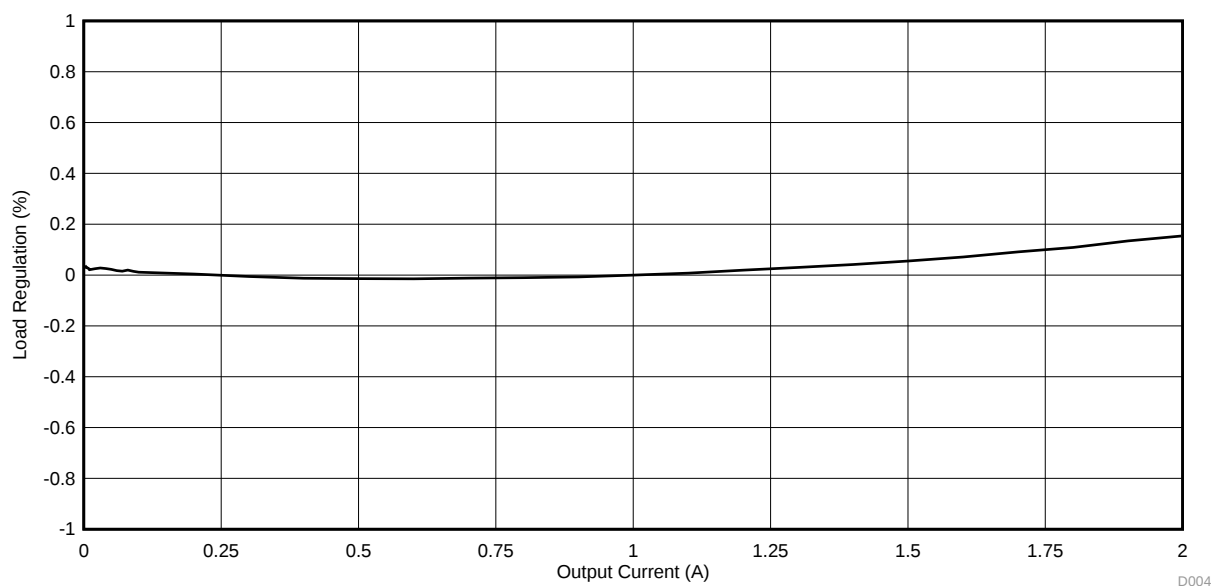
Figure 4. TPS562219EVM-663 Load Regulation, 12 V Input
