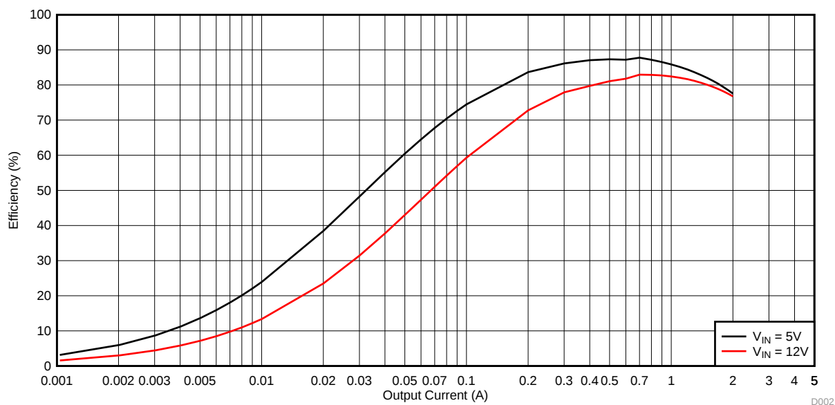
Figure 2. TPS562219EVM-663 Light Load Efficiency
