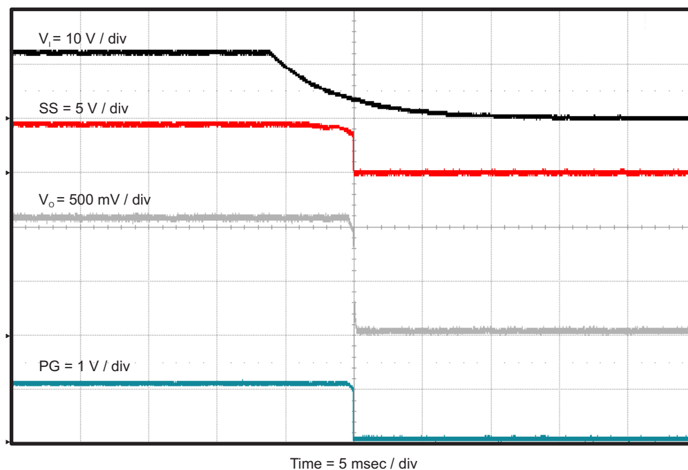
Figure 11. TPS562219EVM-663 Shut-Down Relative to V_{IN}
