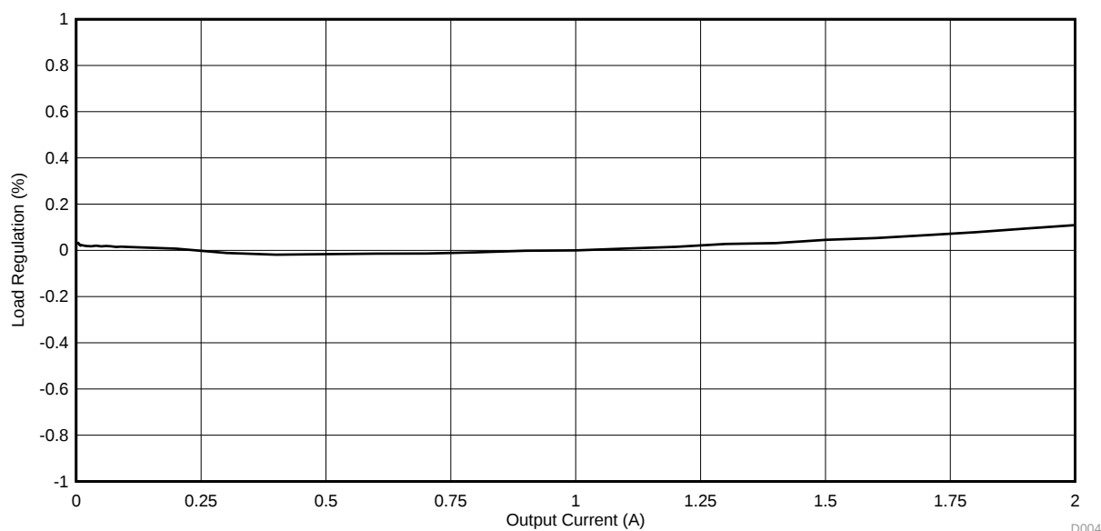
Figure 3. TPS562219EVM-663 Load Regulation, 5 V Input
