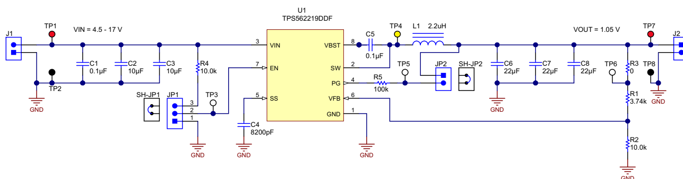
Figure 16. TPS562219EVM-663 Schematic Diagram
