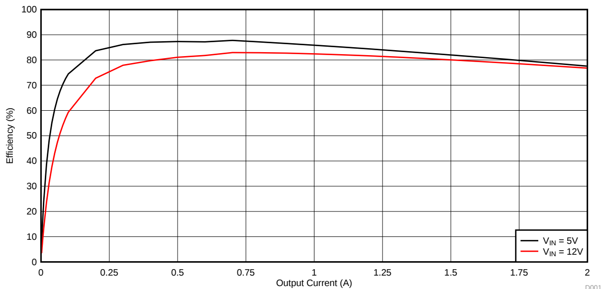
Figure 1. TPS562219EVM-663 Efficiency
