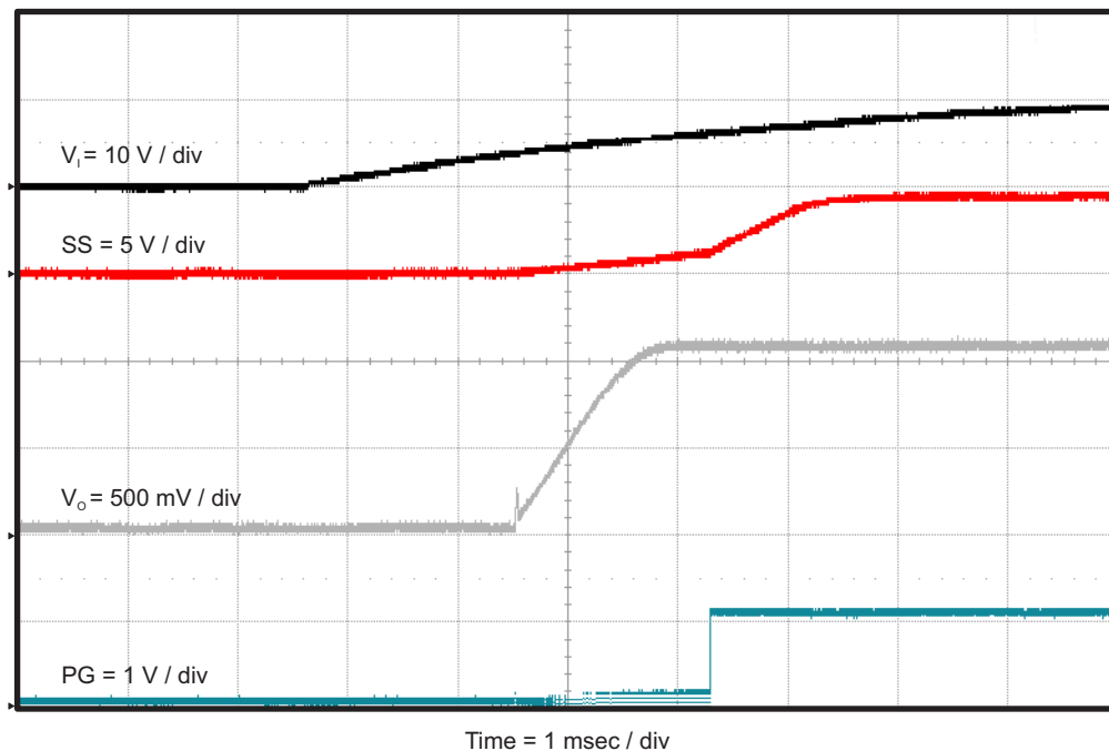
Figure 9. TPS562219EVM-663 Start-Up Relative to V_{IN}
