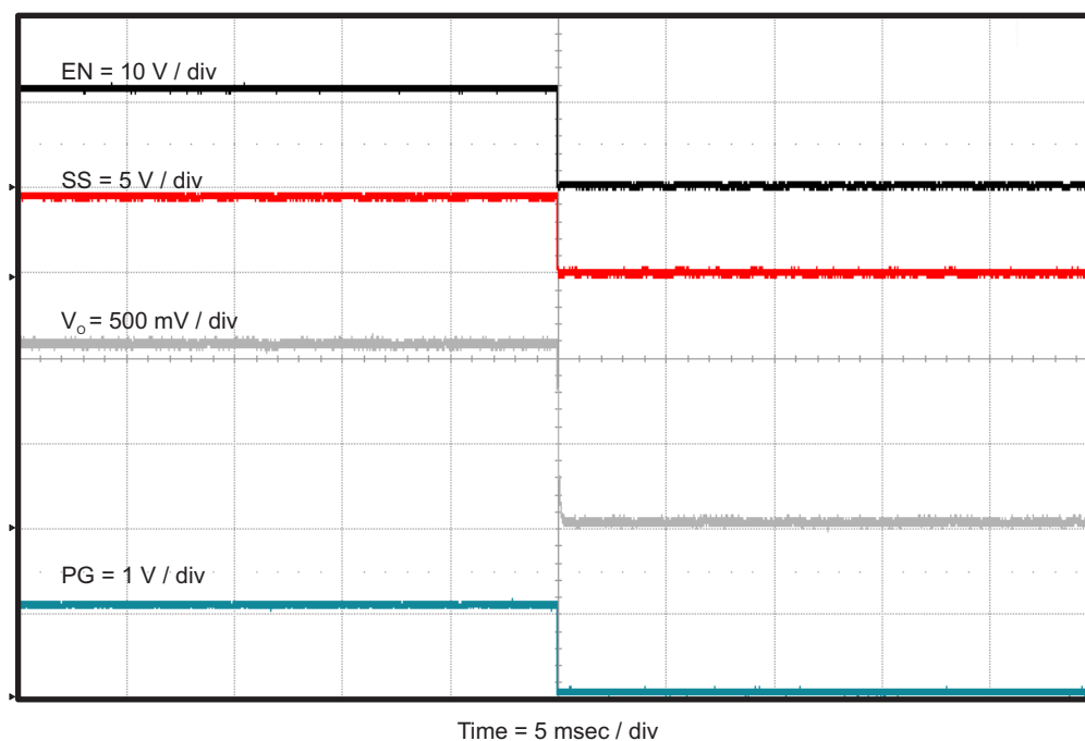
Figure 12. TPS562219EVM-663 Shut-Down Relative to EN
