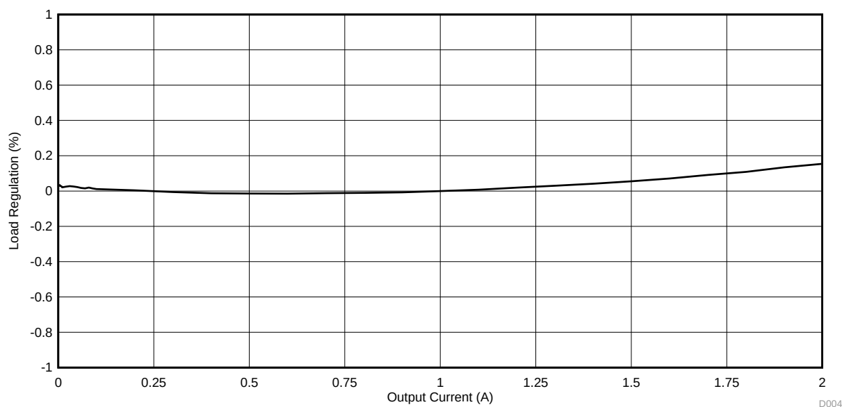
Figure 4. TPS562219AEVM-663 Load Regulation, 12 V Input
