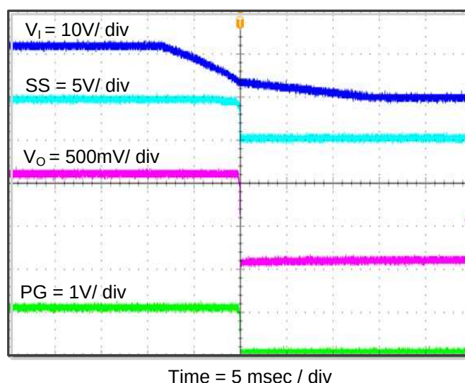
Figure 11. TPS562219AEVM-663 Shut-Down Relative to V_{IN}
