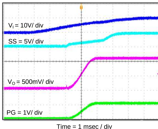
Figure 9. TPS562219AEVM-663 Start-Up Relative to V_{IN}
