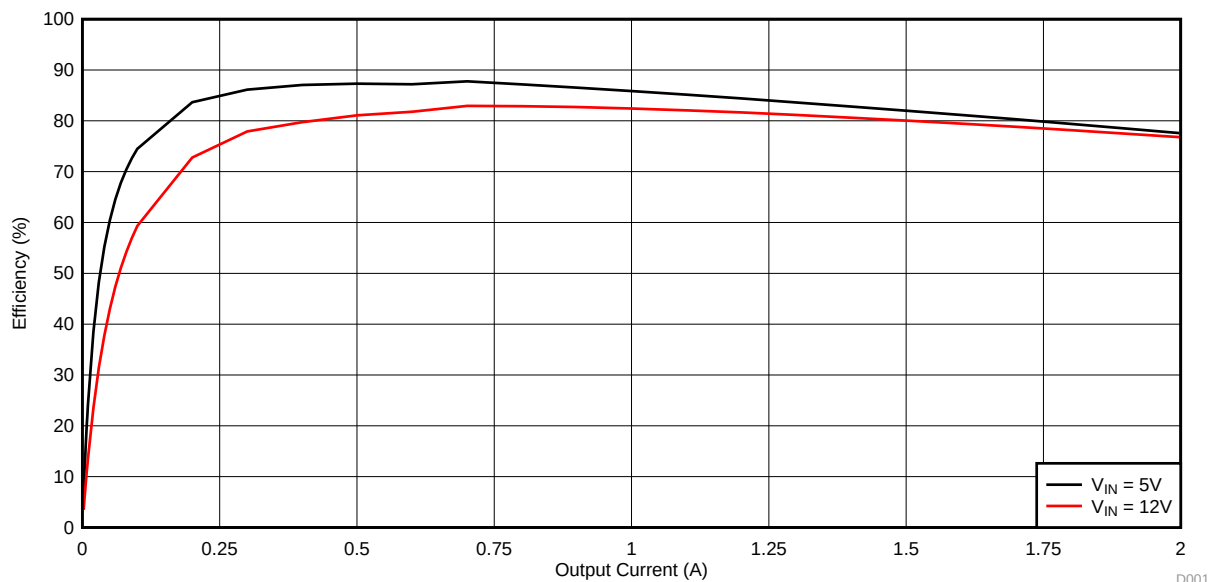
Figure 1. TPS562219AEVM-663 Efficiency
