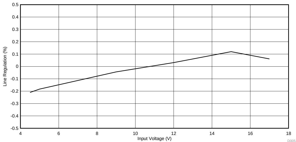
Figure 5. TPS562219AEVM-663 Line Regulation
