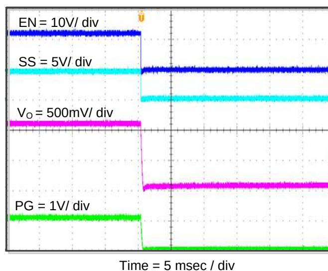
Figure 12. TPS562219AEVM-663 Shut-Down Relative to EN
