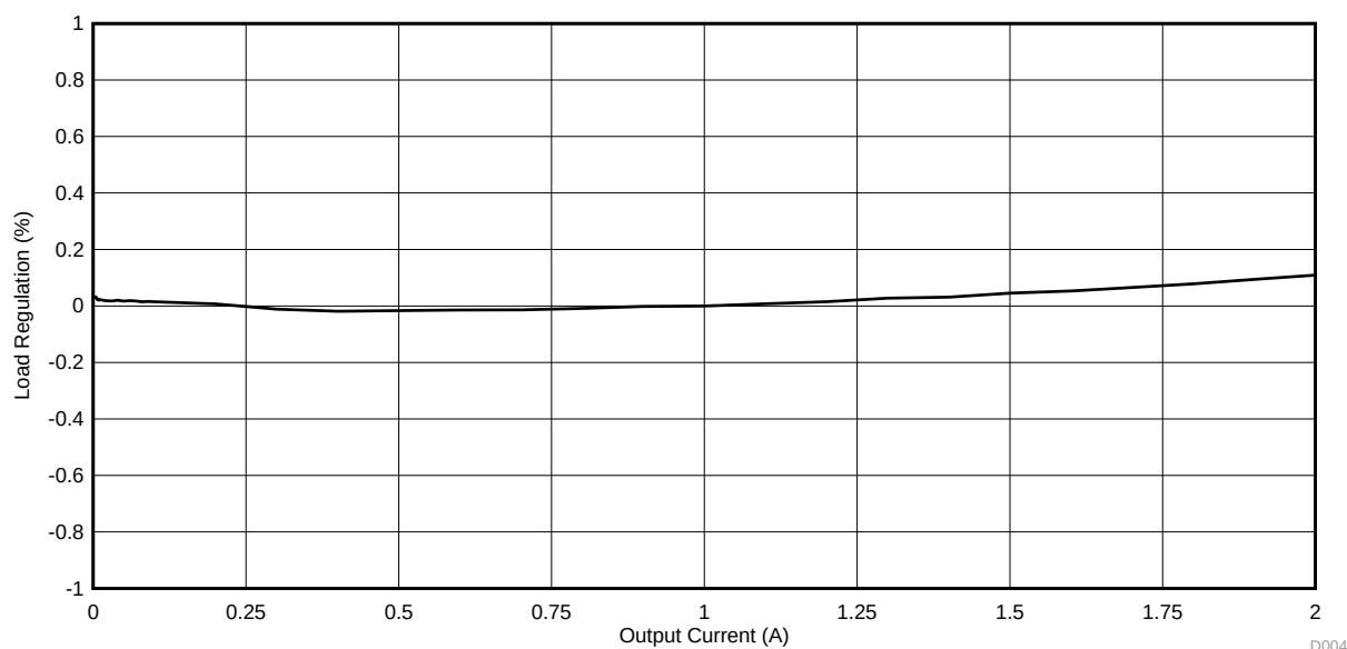
Figure 3. TPS562219AEVM-663 Load Regulation, 5 V Input
