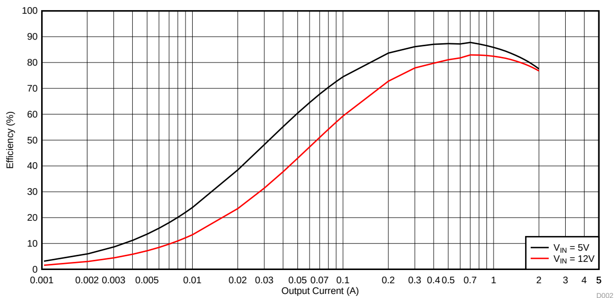
Figure 2. TPS562219AEVM-663 Light Load Efficiency
