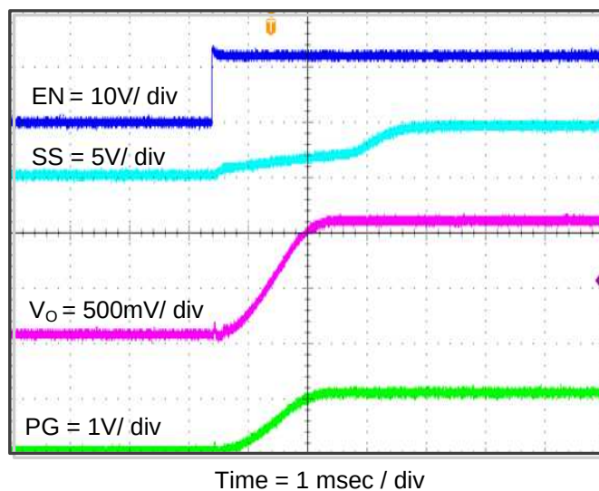
Figure 10. TPS562219AEVM-663 Start-Up Relative to EN
