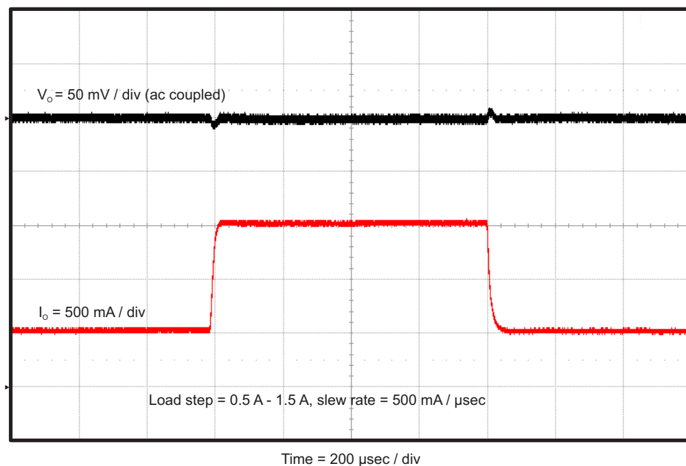
Figure 6. TPS562219AEVM-663 Load Transient Response, 25% to 75% Load Step
