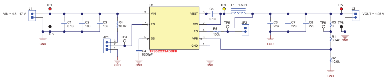
Figure 16. TPS562219AEM-663 Schematic Diagram
