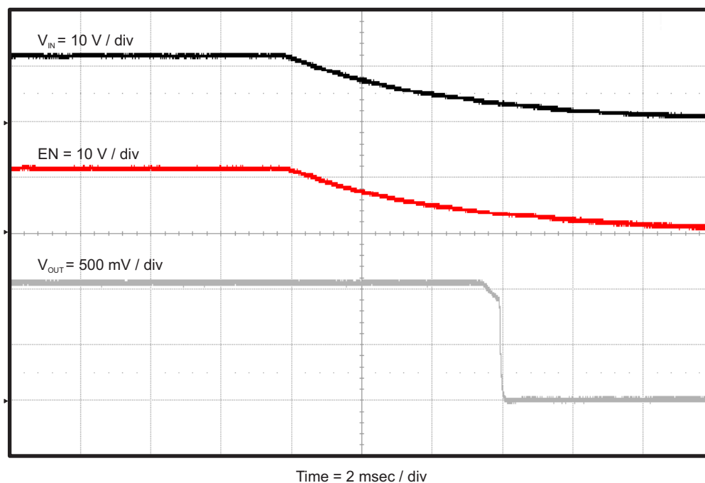
Figure 10. TPS562209EVM-601 Shut-Down Relative to V_{IN}
