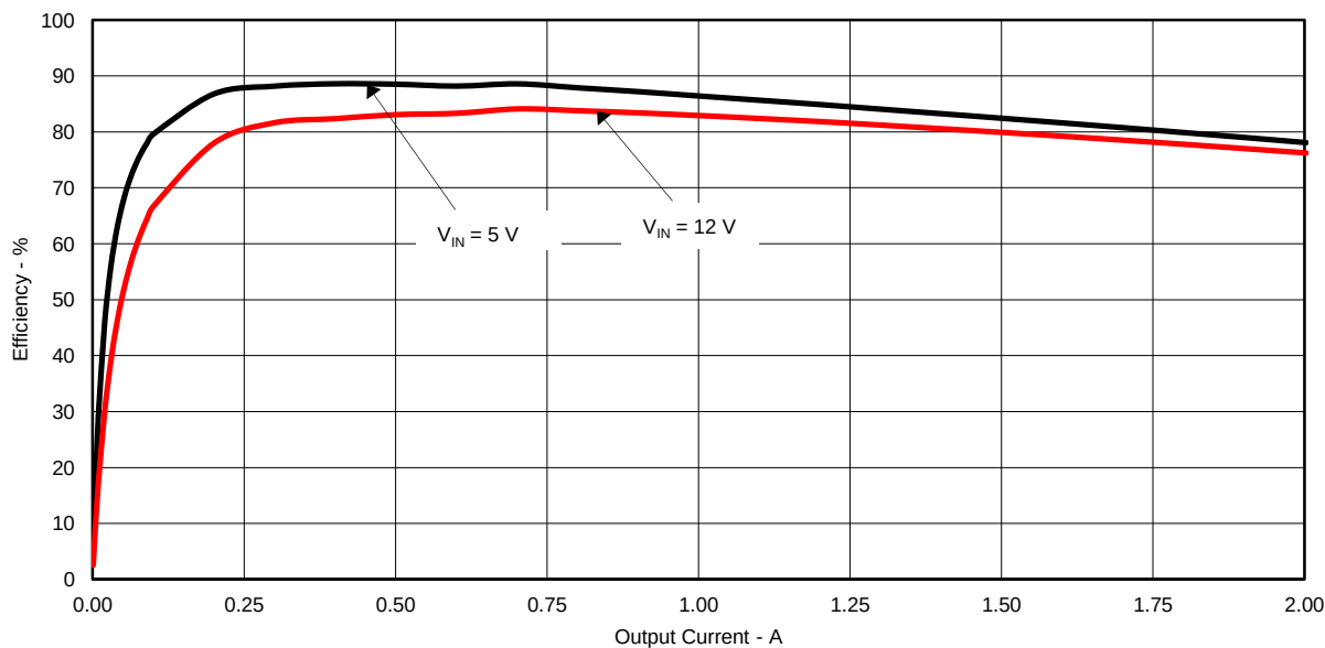
Figure 1. TPS562209EVM-601 Efficiency
