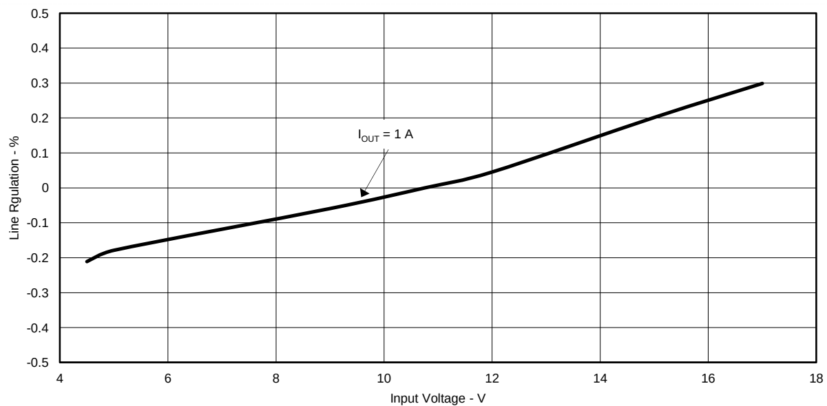
Figure 4. TPS562209EVM-601 Line Regulation
