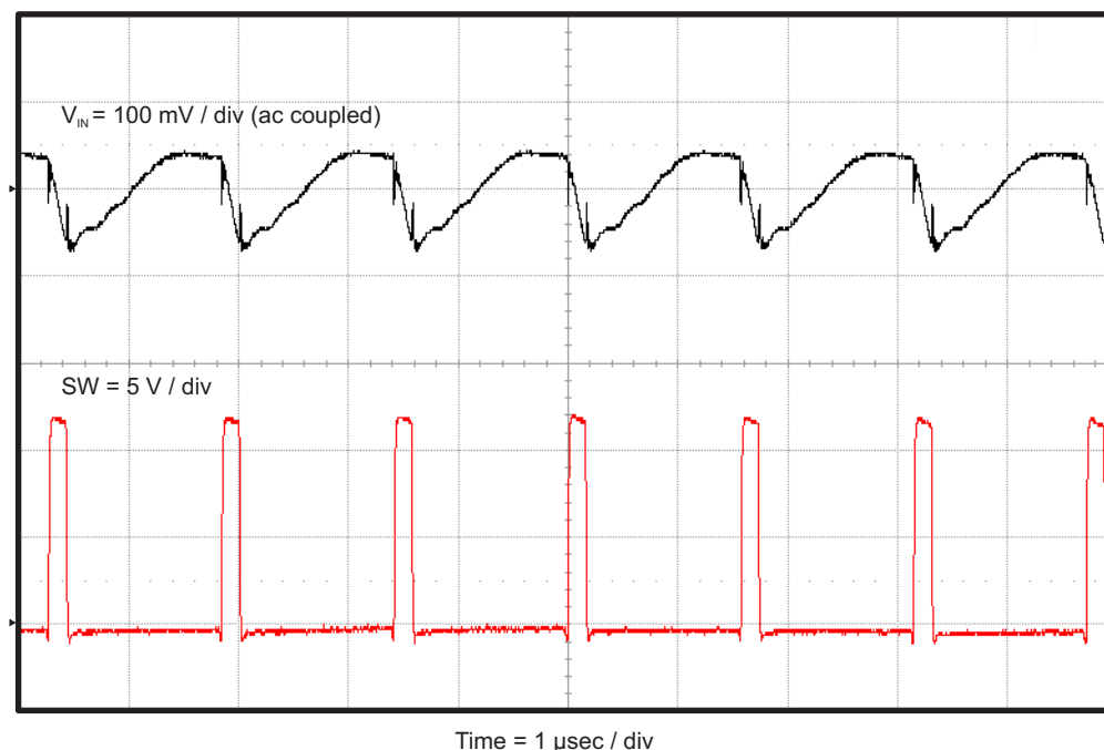
Figure 7. TPS562209EVM-601 Input Voltage Ripple, I_{OUT} = 2 A
