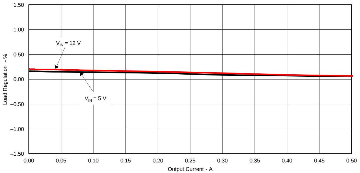
Figure 3. TPS562209EVM-601 Load Regulation
