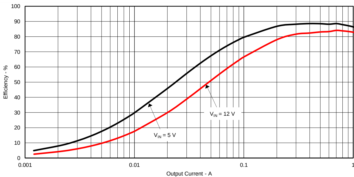
Figure 2. TPS562209EVM-601 Light Load Efficiency
