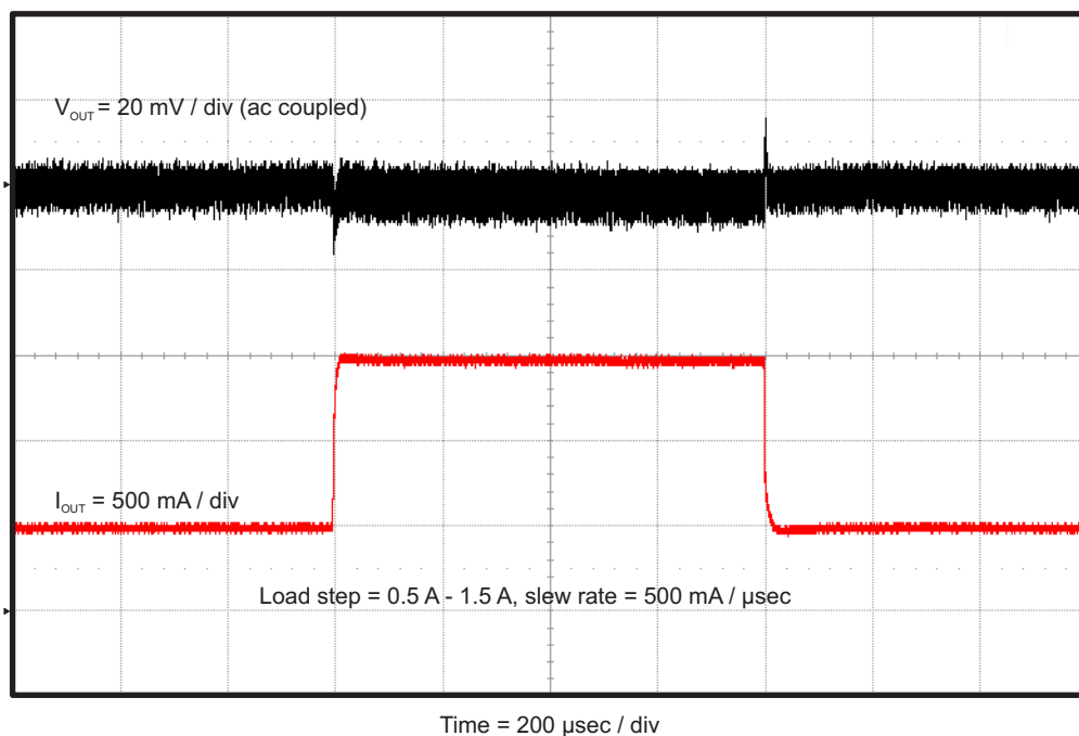
Figure 5. TPS562209EVM-601 Load Transient Response, 25% to 75% Load Step
