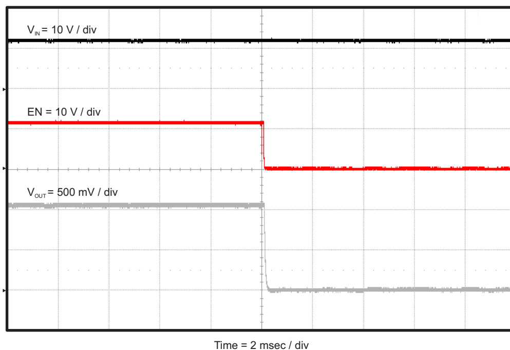
Figure 11. TPS562209EVM-601 Shut-Down Relative to EN
