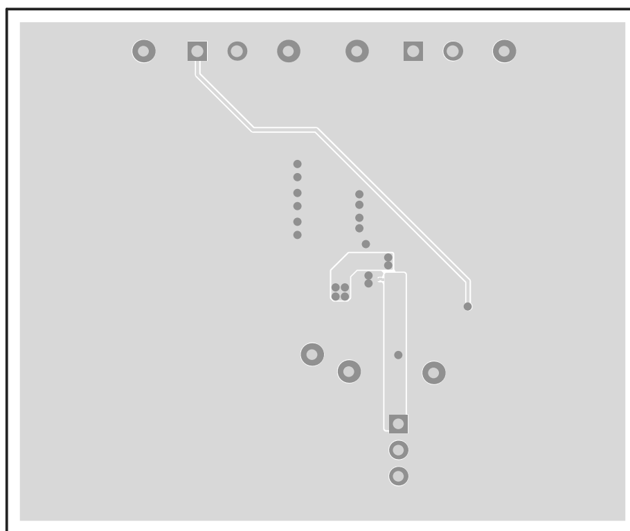
Figure 13. Bottom Layer
