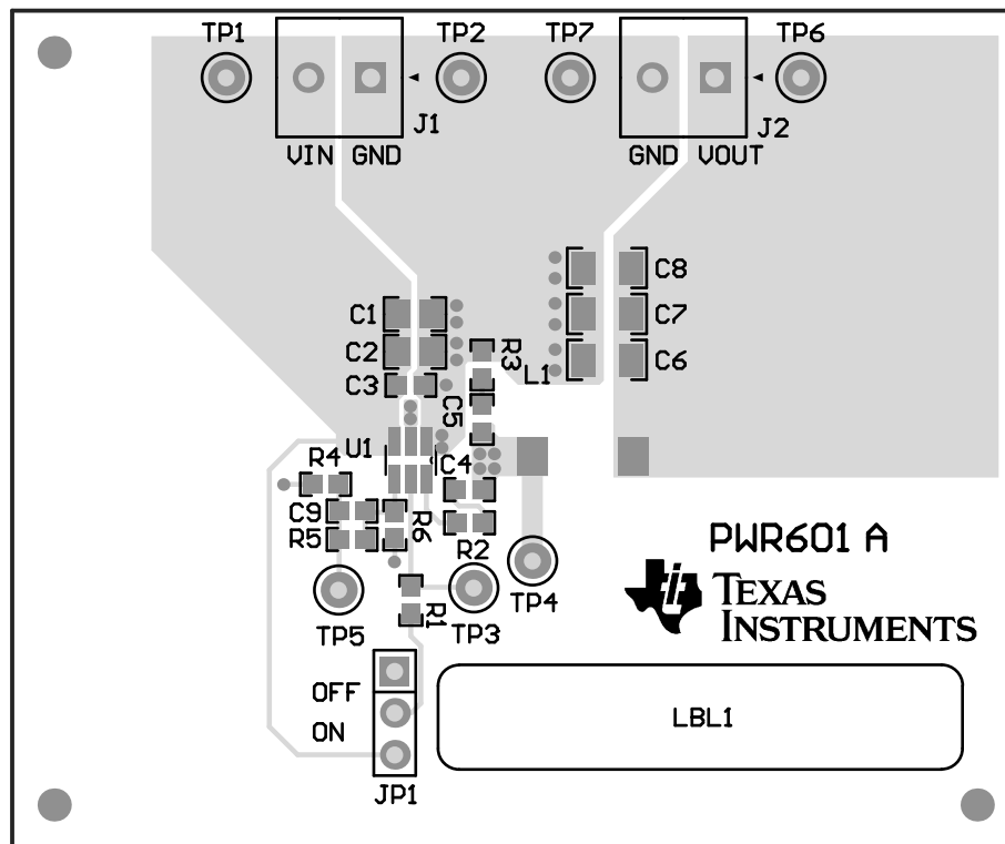
Figure 12. Top Assembly
