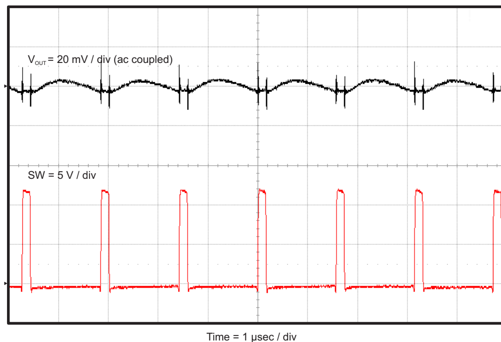
Figure 6. TPS562209EVM-601 Output Voltage Ripple, I_{OUT} = 2 A
