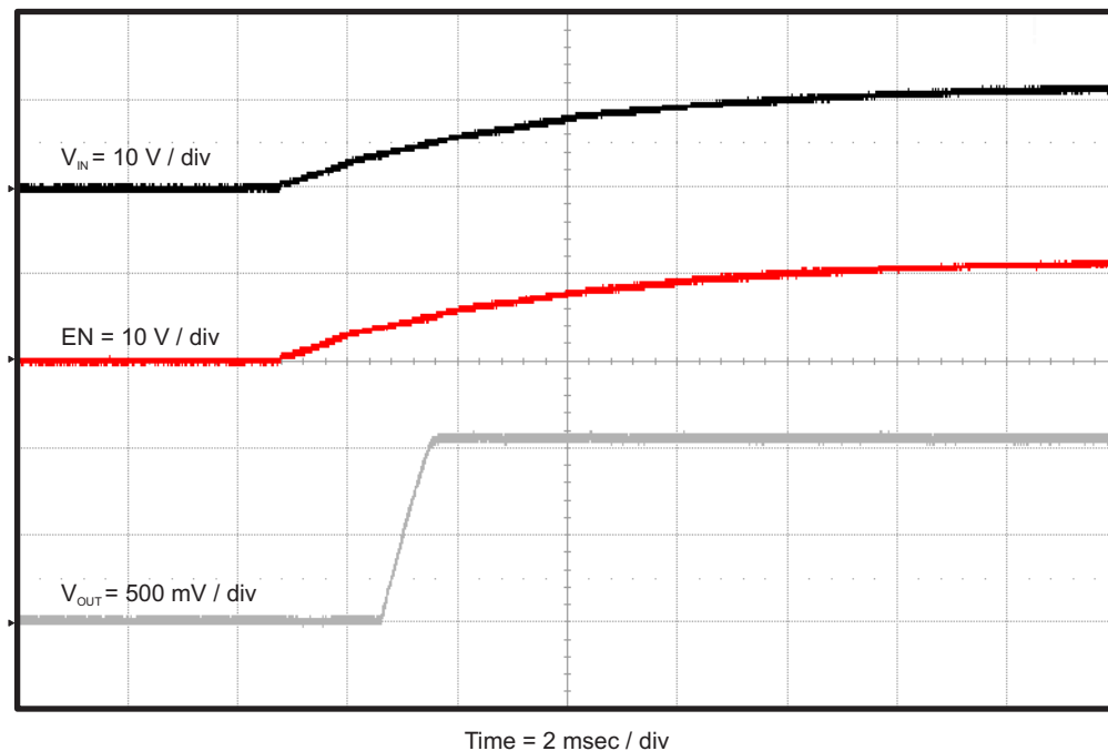
Figure 8. TPS562209EVM-601 Start-Up Relative to V_{IN}
