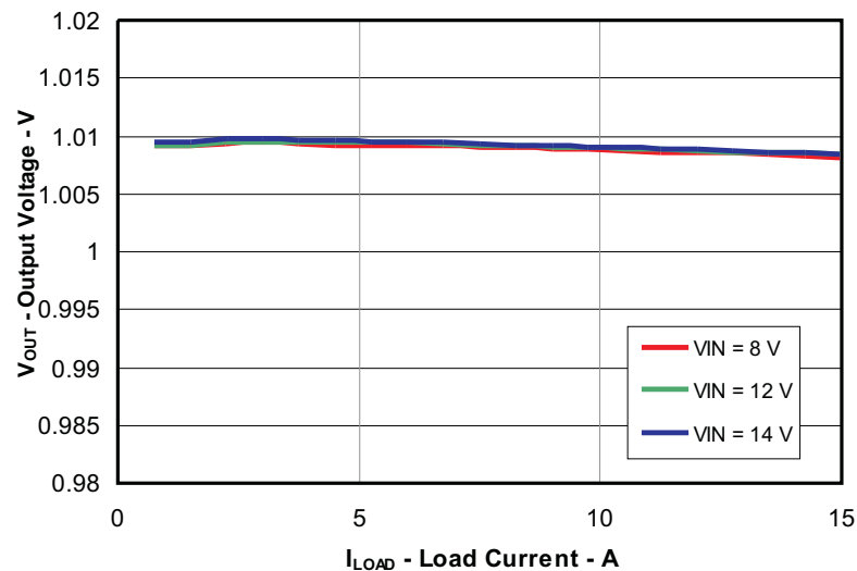
Figure 6. Load Regulation
