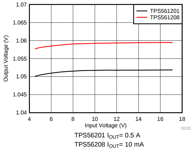
Figure 20. Line Regulation
