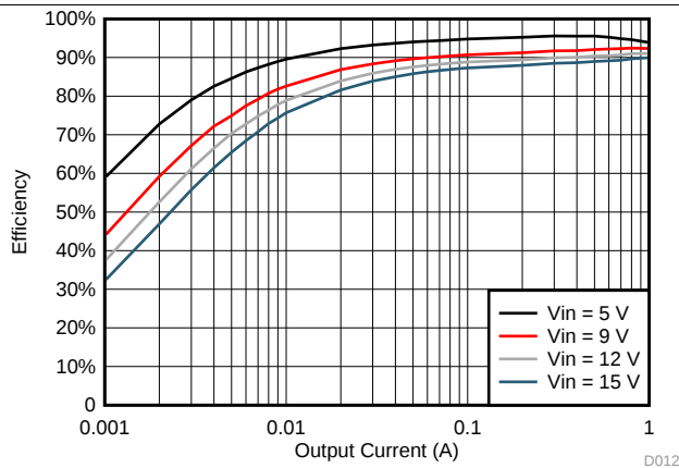
Figure 9. TPS561201 V_{OUT} = 1.05\text{ V} Efficiency, L = 2.2\text{ }\mu\text{H}
