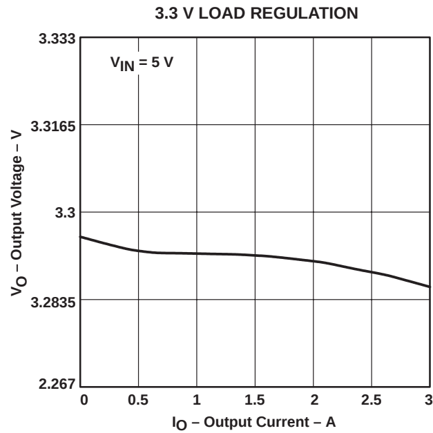
Figure 2–2. SLVP133 Measured Load Regulation 3.3-V Output
